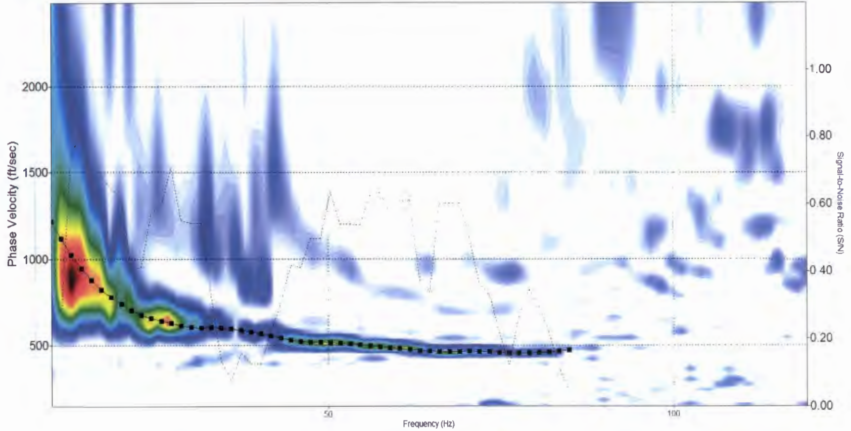
Line B Dispersion Curve (Record # = 80) (Mid-Station # = 127.5)
