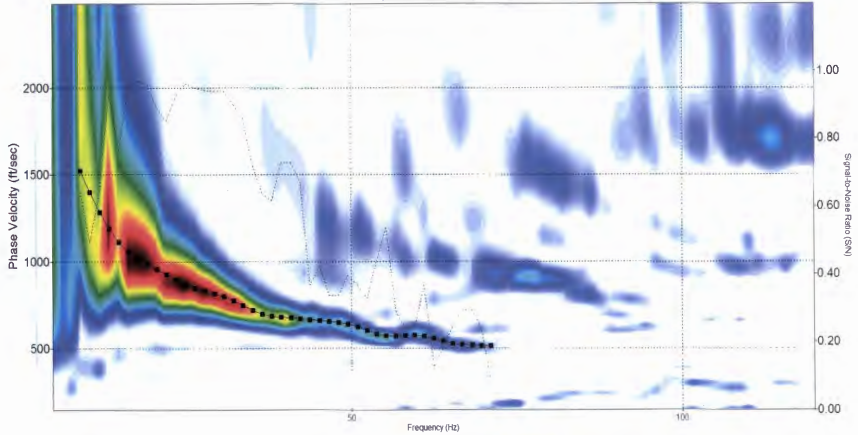
Line A Dispersion Curve (Record # = 1) (Mid-Station # = 111.5)
