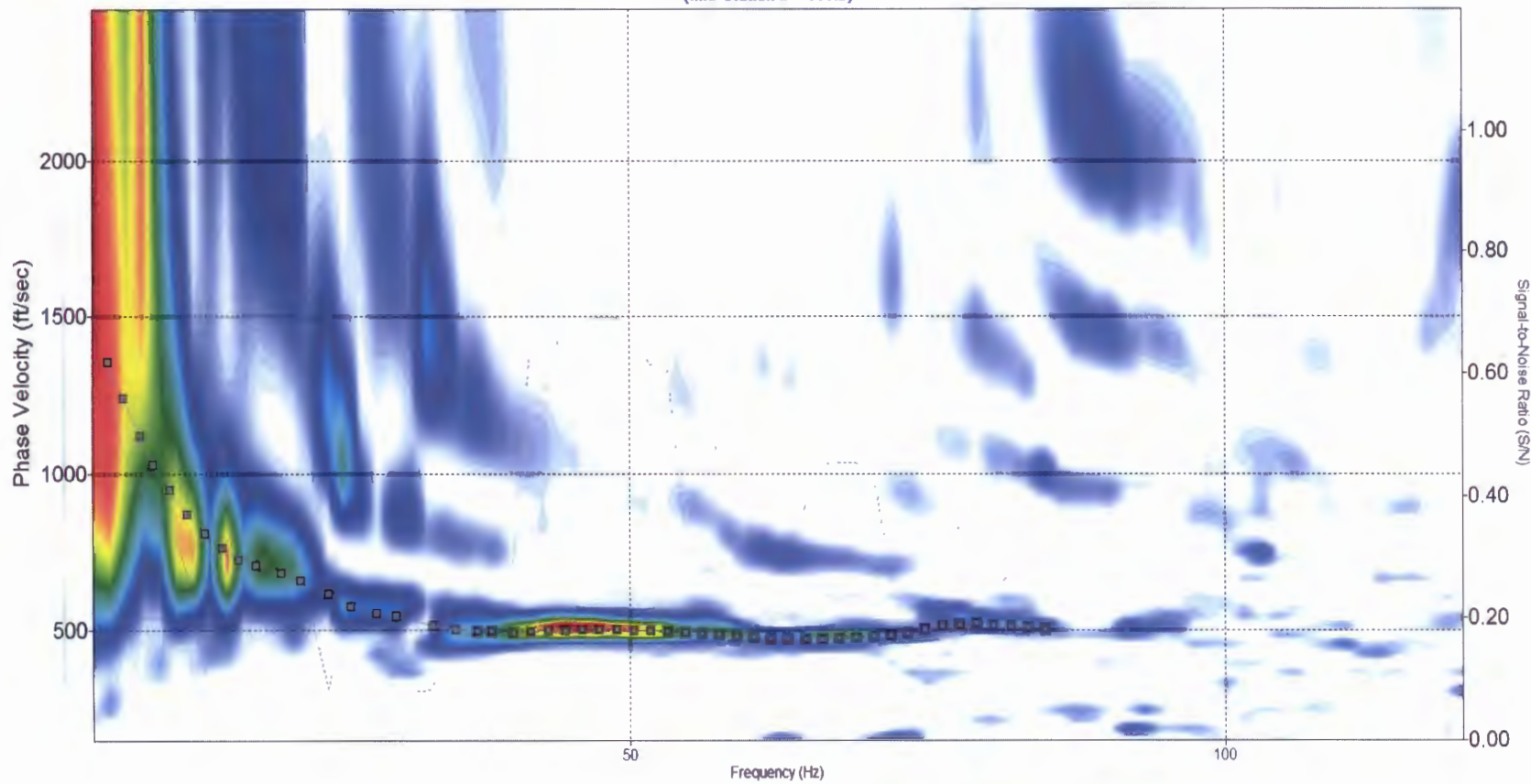
Line E Dispersion Curve (Record # = 288) (Mid-Station # = 111.5)
