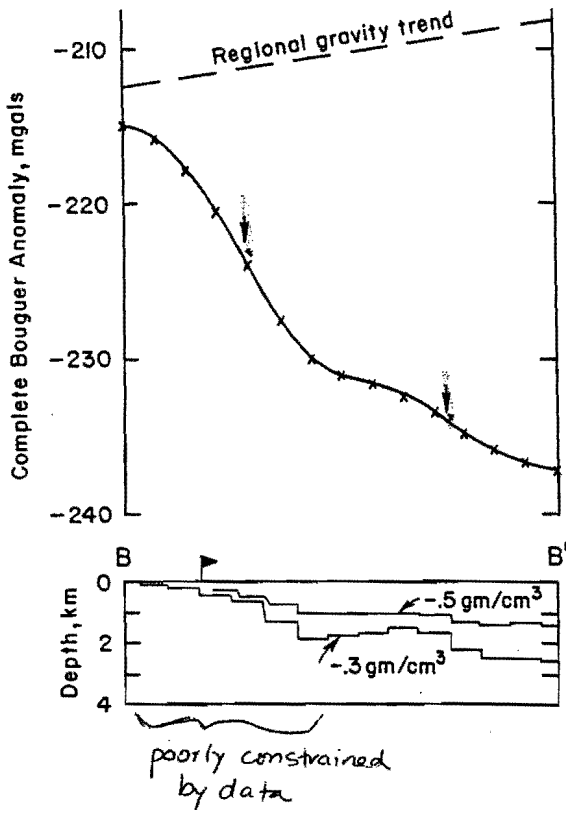
Figure 3. Profile B-B' (see fig. 1 for location). Lower graph shows depth to base of low-density graben fill, calculated from the gravity data for two different density contrasts ( -0.3 and -0.5 \text{ gm/cm}^3 , as indicated). Horizontal and vertical scales in the derived graben-fill models are the same and are indicated on the "depth" ordinate of the lower figure. Flags show the approximate limits of graben fill as determined from geologic mapping. In the upper figure, the Bouguer anomaly profile (fig. 1) is shown by solid line, and gravity effect calculated from the -0.3 \text{ gm/cm}^3 model is indicated by "x". (Fit of the -0.5 \text{ gm/cm}^3 model is generally better.) Vertical arrows show inflection points, as determined from Figure 6.
