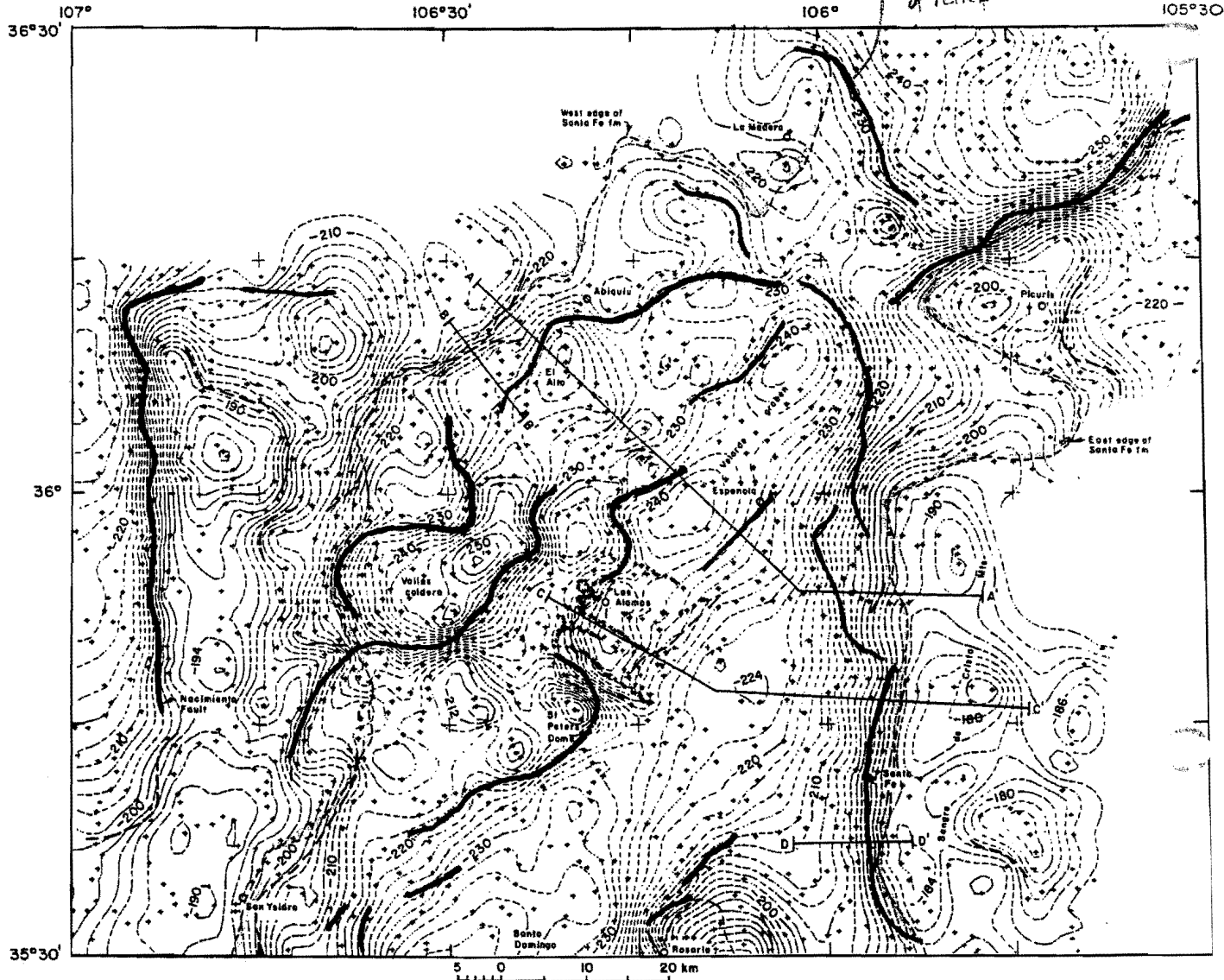
Figure 1. Complete Bouguer-anomaly gravity map centered on the Española basin section of the Rio Grande rift. Contour interval 2 mgals; reduction density 2.5 \text{ gm/cm}^3 . Gravity stations indicated by "+". Hachures indicate local closed minima. Limit of Santa Fe Group and related graben-filling rocks shown by fine dashed line. Locus of principal gravity inflection points shown by heavy dashed lines (from fig. 6). Profile bars show locations of profiles A, B, C and D (figs. 2-5).
