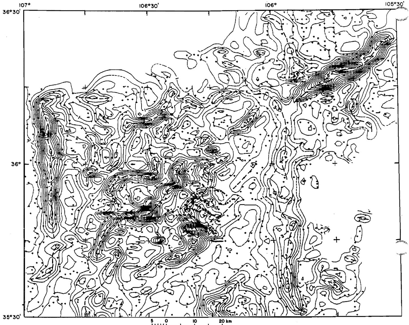
Figure 6. Gravity gradient (amplitude of horizontal component of gravity gradient (contour interval = 0.5 mgals/km)). Heavy dashed lines show significant maxima marking the locus of gravity-anomaly inflection points, and by inference, the approximate location of major faults or steep lithologic contacts.
