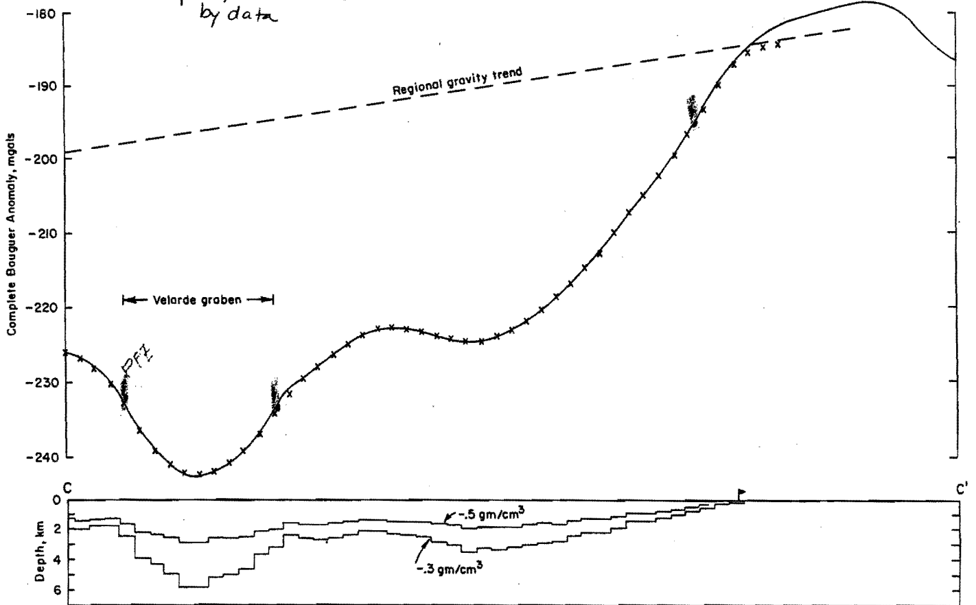
Figure 4. Profile C-C' (see fig. 1 for location). Lower graph shows depth to base of low-density graben fill, calculated from the gravity data for two different density contrasts ( -0.3 and -0.5 \text{ gm/cm}^3 , as indicated). Horizontal and vertical scales in the derived graben-fill models are the same and are indicated on the "depth" ordinate of the lower figure. Flags show the approximate limits of graben fill as determined from geologic mapping. In the upper figure, the Bouguer anomaly profile (fig. 1) is shown by solid line, and gravity effect calculated from the -0.3 \text{ gm/cm}^3 model is indicated by "x". (Fit of the -0.5 \text{ gm/cm}^3 model is generally better.) Vertical arrows show inflection points, as determined from Figure 6.
