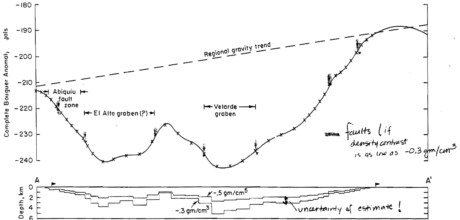
Figure 2. Profile A-A' (see fig. 1 for location). Lower graph shows depth to base of low-density graben fill, calculated from the gravity data for two different density contrasts ( -0.3 and -0.5 gm/cm 3 , as indicated). Horizontal and vertical scales in the derived graben-fill models are the same and are indicated on the "depth" ordinate of the lower figure. Flags show the approximate limits of graben fill as determined from geologic mapping. In the upper figure, the Bouguer anomaly profile (fig. 1) is shown by solid line, and gravity effect calculated from the -0.3 gm/cm 3 model is indicated by "x". (Fit of the -0.5 gm/cm 3 model is generally better.) Vertical arrows show inflection points, as determined from Figure 6.
