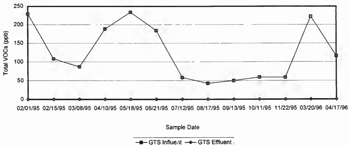
Figure 5 Total VOCs GTS Influent vs. Effluent
