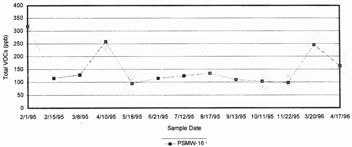
Figure 2 Total VOCs at PSMW-16
