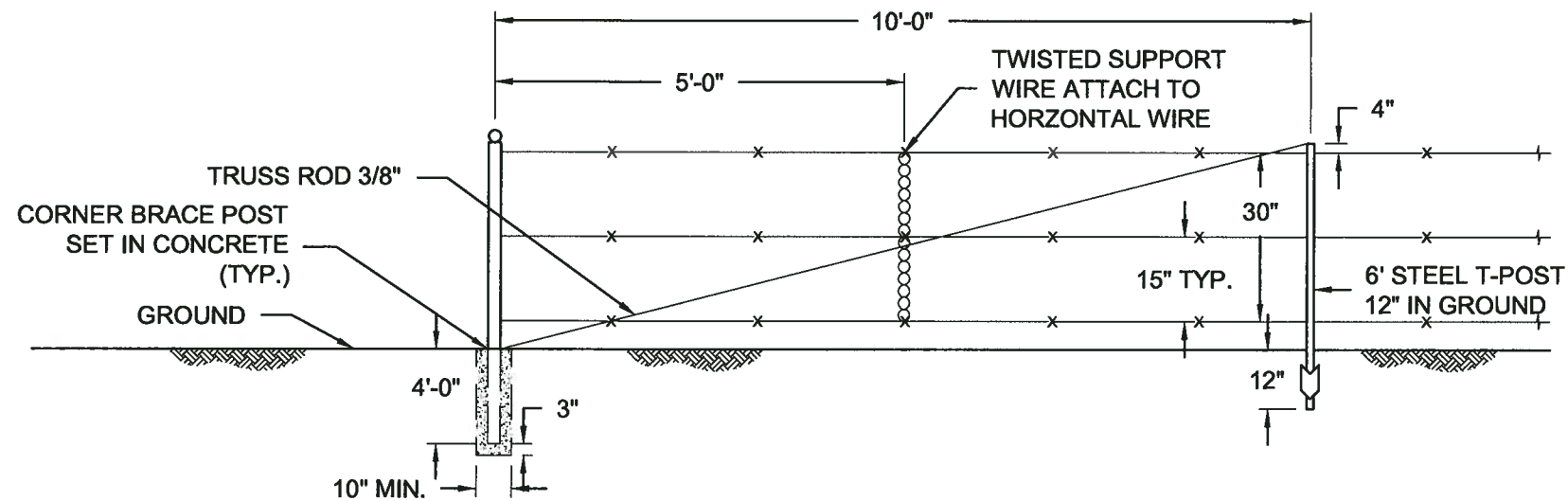
1 ADMINISTRATIVE CONTROL FENCE AND GATE (See Note) 2 DETAIL NTS
