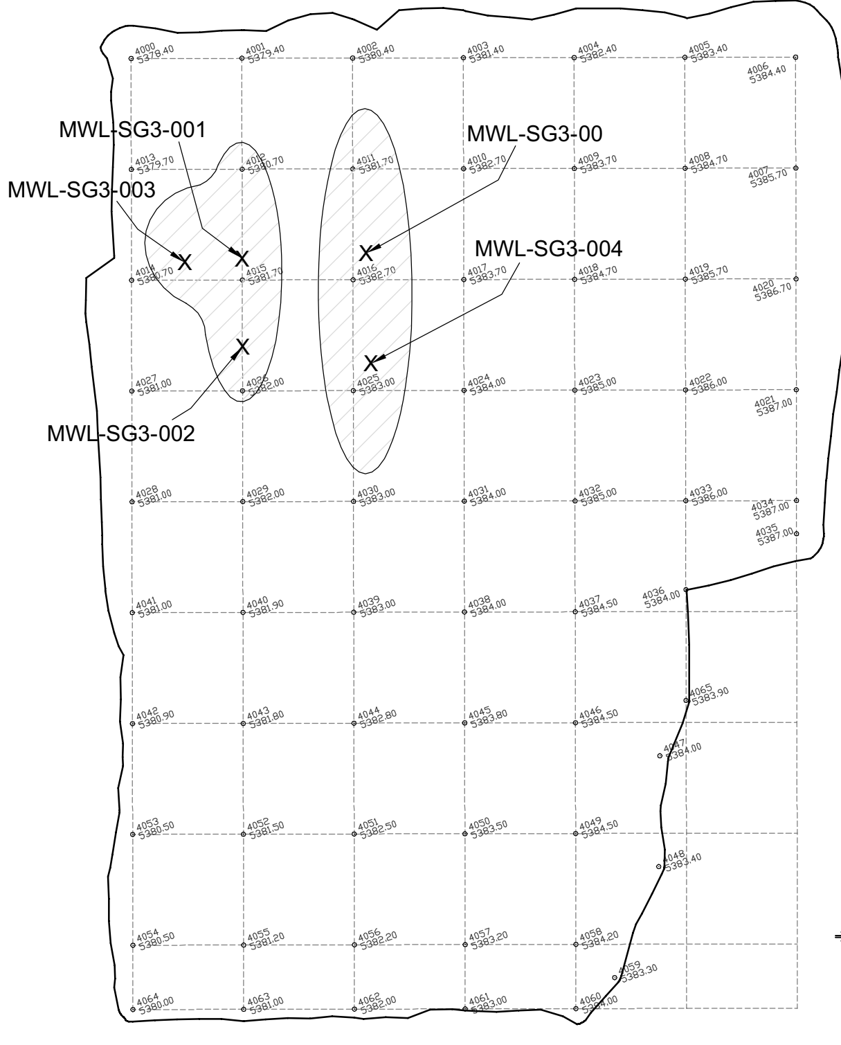
Figure 8 Mixed Waste Landfill Subgrade Lift 3 Map
