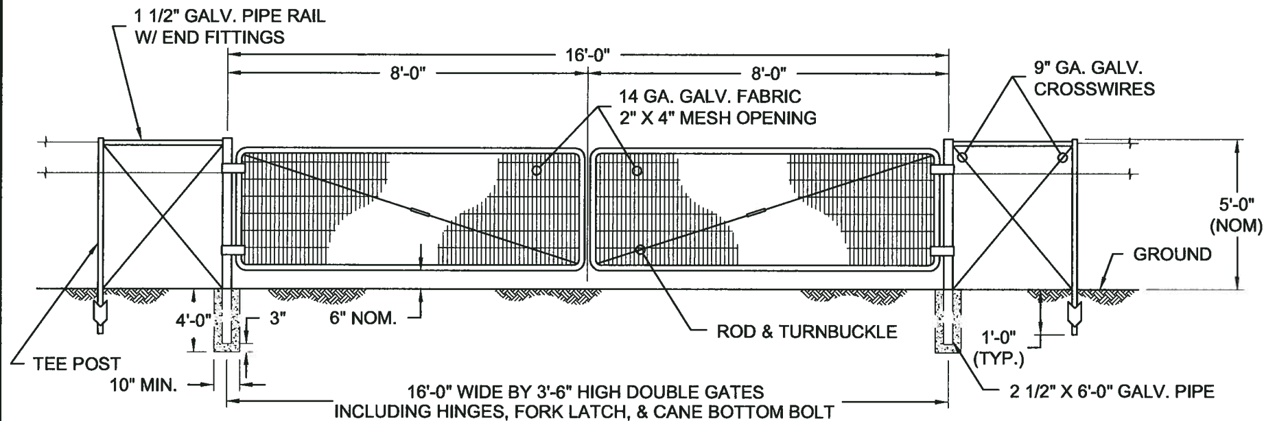
2 ADMINISTRATIVE CONTROL FENCE AND GATE (See Note) 2 DETAIL NTS
