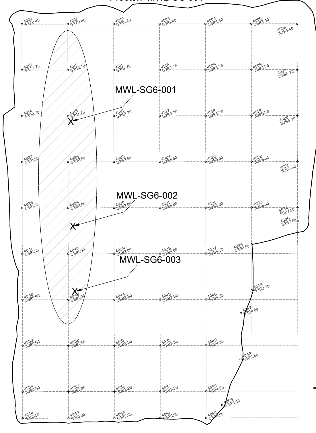
Figure 11 Mixed Waste Landfill Subgrade Lift 6 Map
