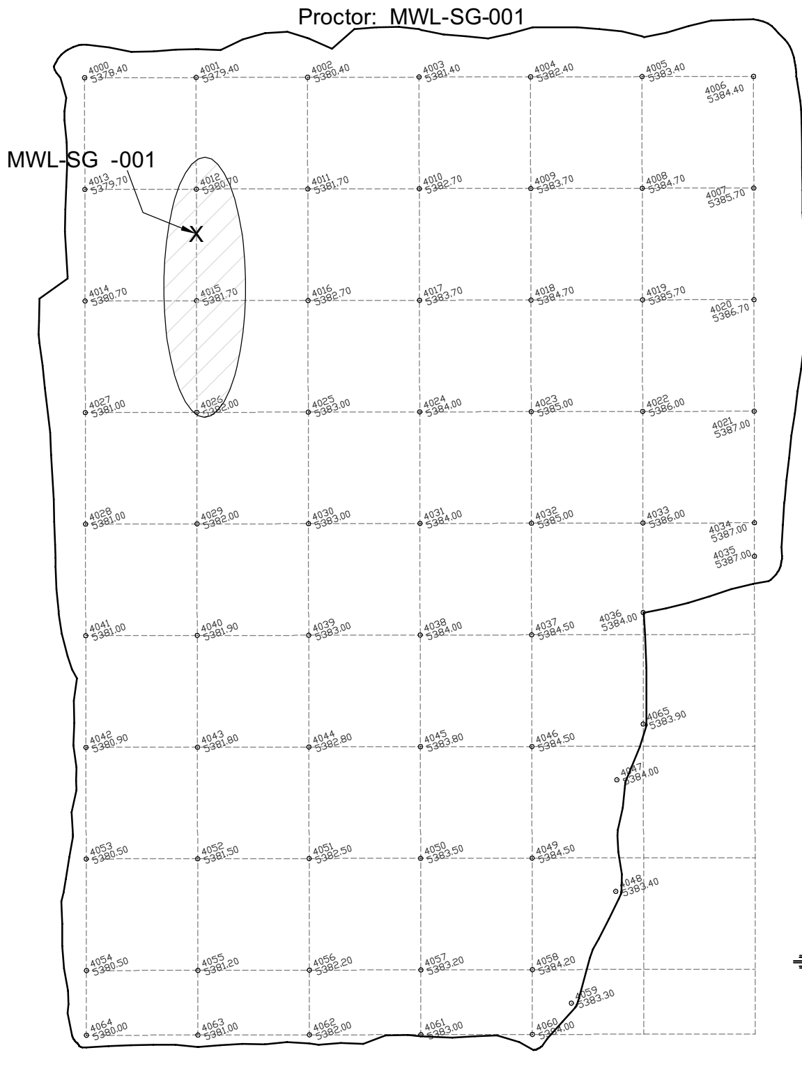
Figure 10 Mixed Waste Landfill Subgrade Lift 5 Map
