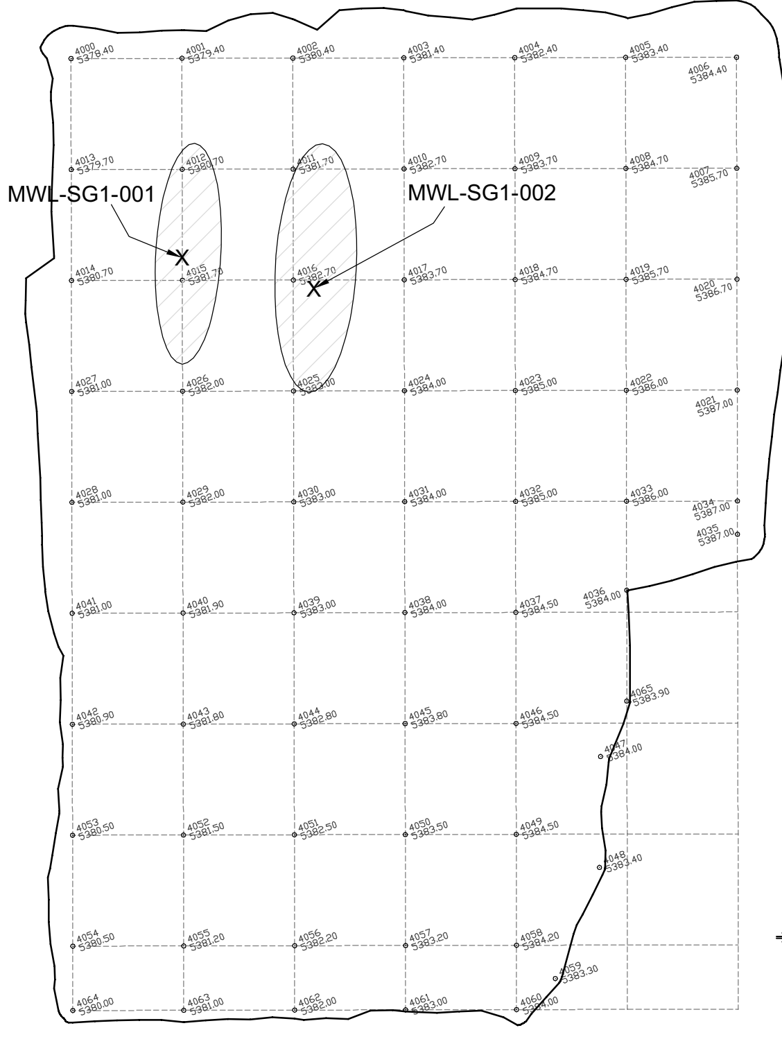
Figure 6 Mixed Waste Landfill Subgrade Lift 1 Map
