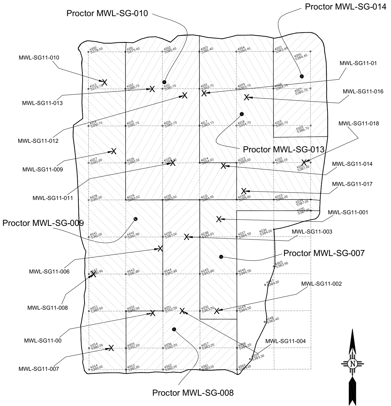
Figure 16 Mixed Waste Landfill Subgrade Lift 11 Map
