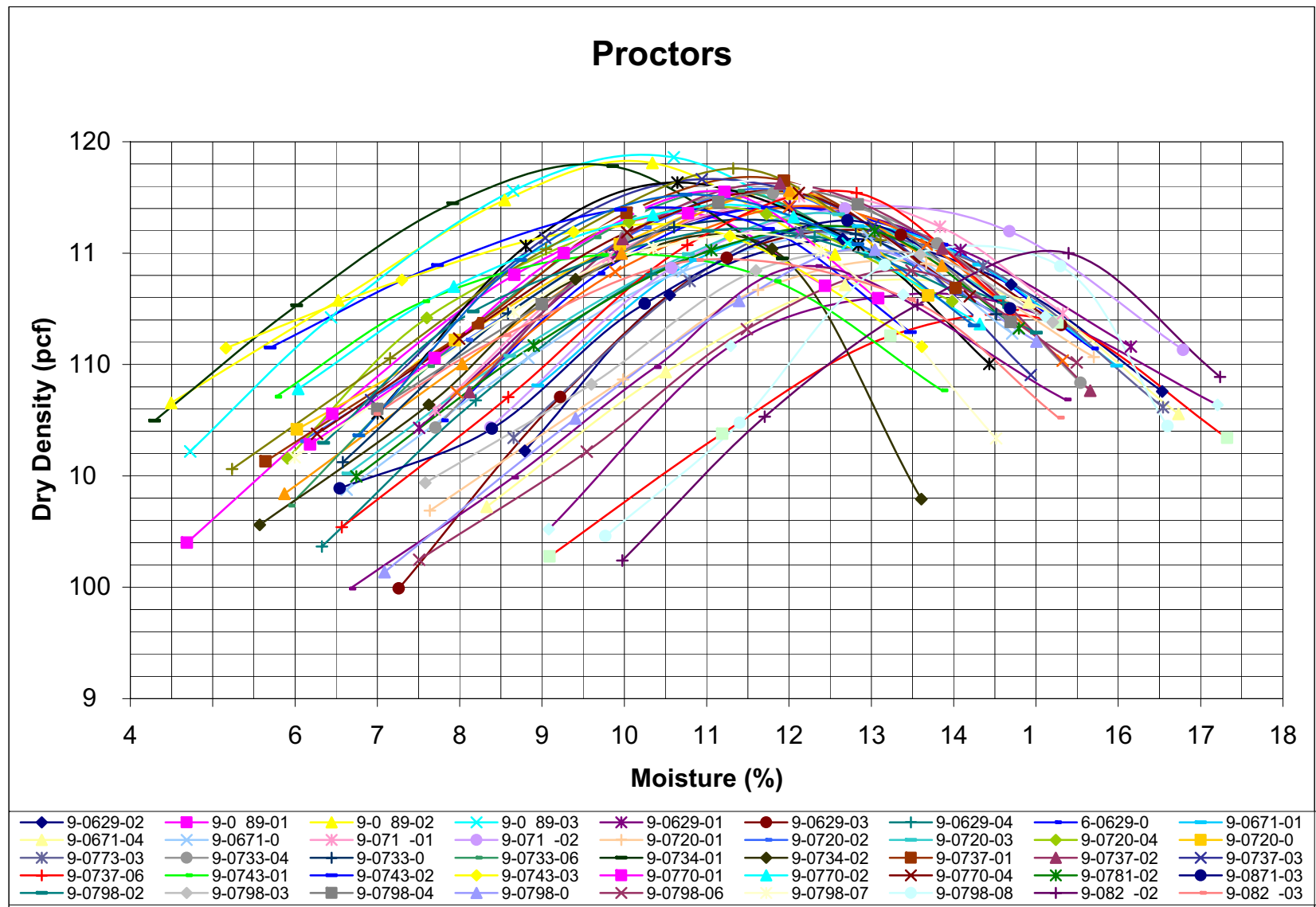
Figure 20. Graphical Representation of all MWL Alternative Cover Standard Proctor Results
