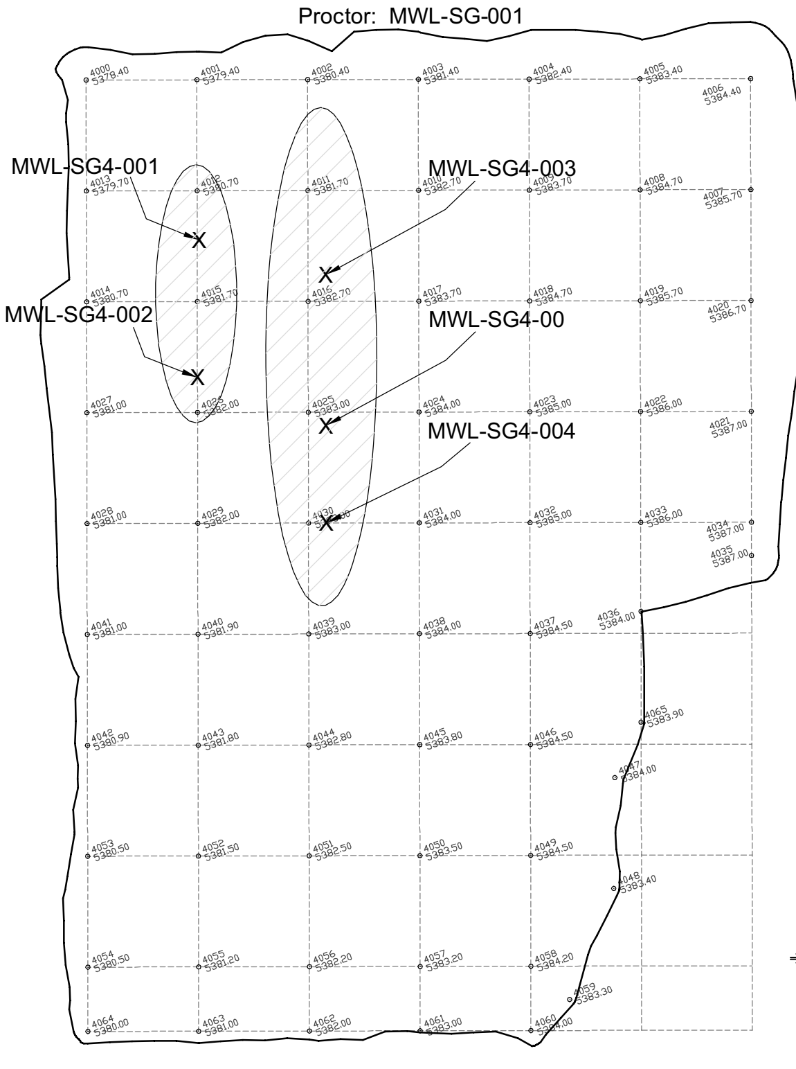
Figure 9 Mixed Waste Landfill Subgrade Lift 4 Map
