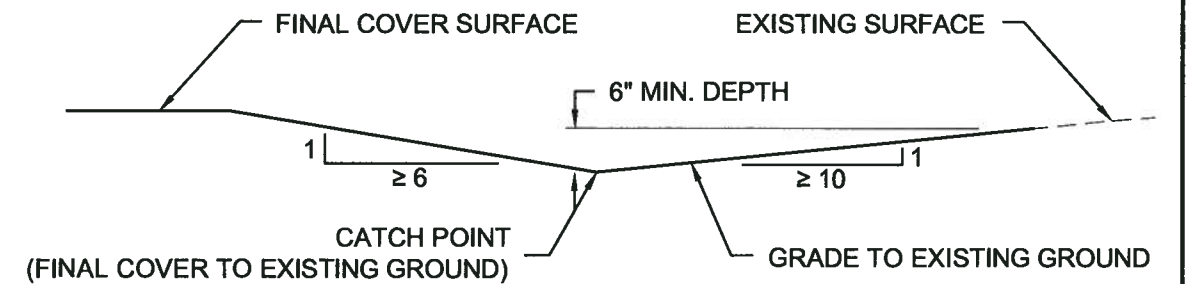
3 TYPICAL DRAINAGE SWALE SECTION 2 DETAIL NTS
