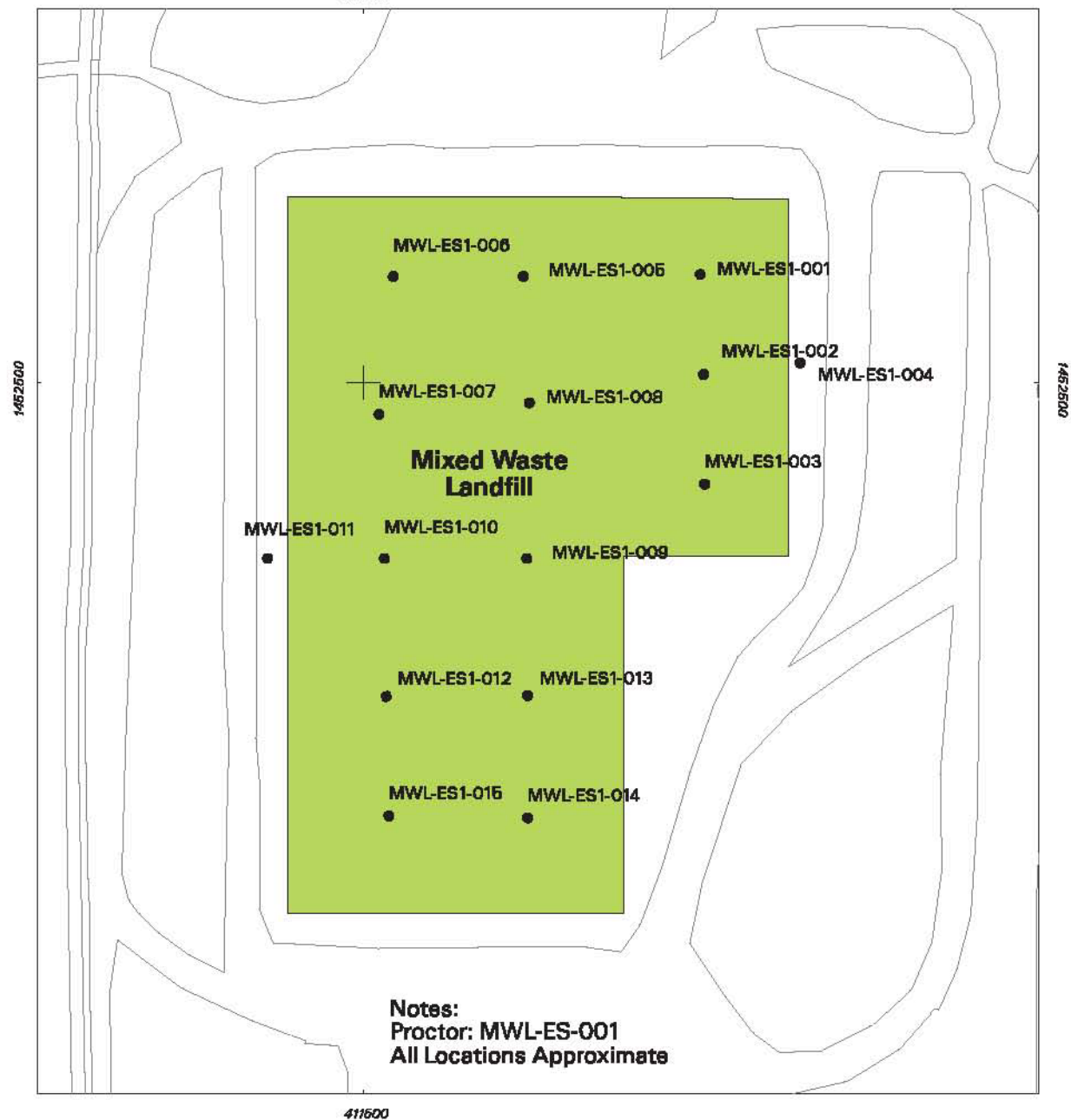
Figure 5 Mixed Waste Landfill 2006 Existing Surface Map
