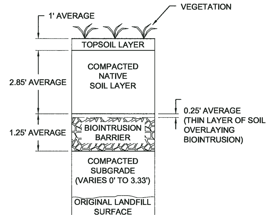
4 GENERALIZED COVER CROSS SECTION 2 DETAIL NTS
