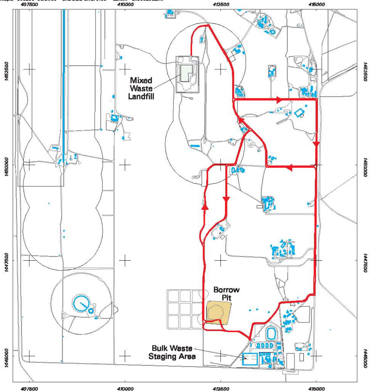
Figure 3 Location of the Mixed Waste Landfill, Borrow Pit, Bulk Waste Staging Area, and Haul Routes
