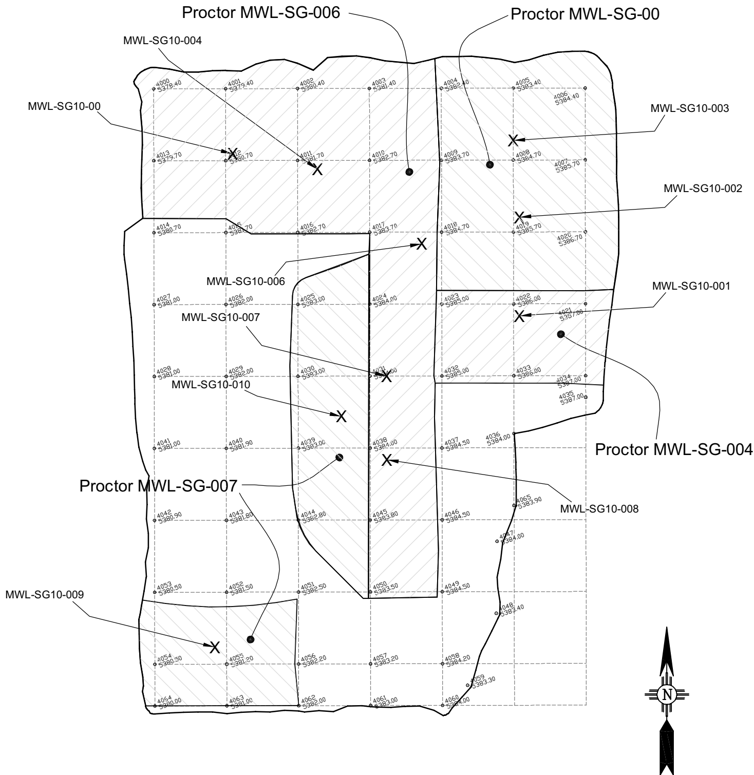
Figure 15 Mixed Waste Landfill Subgrade Lift 10 Map
