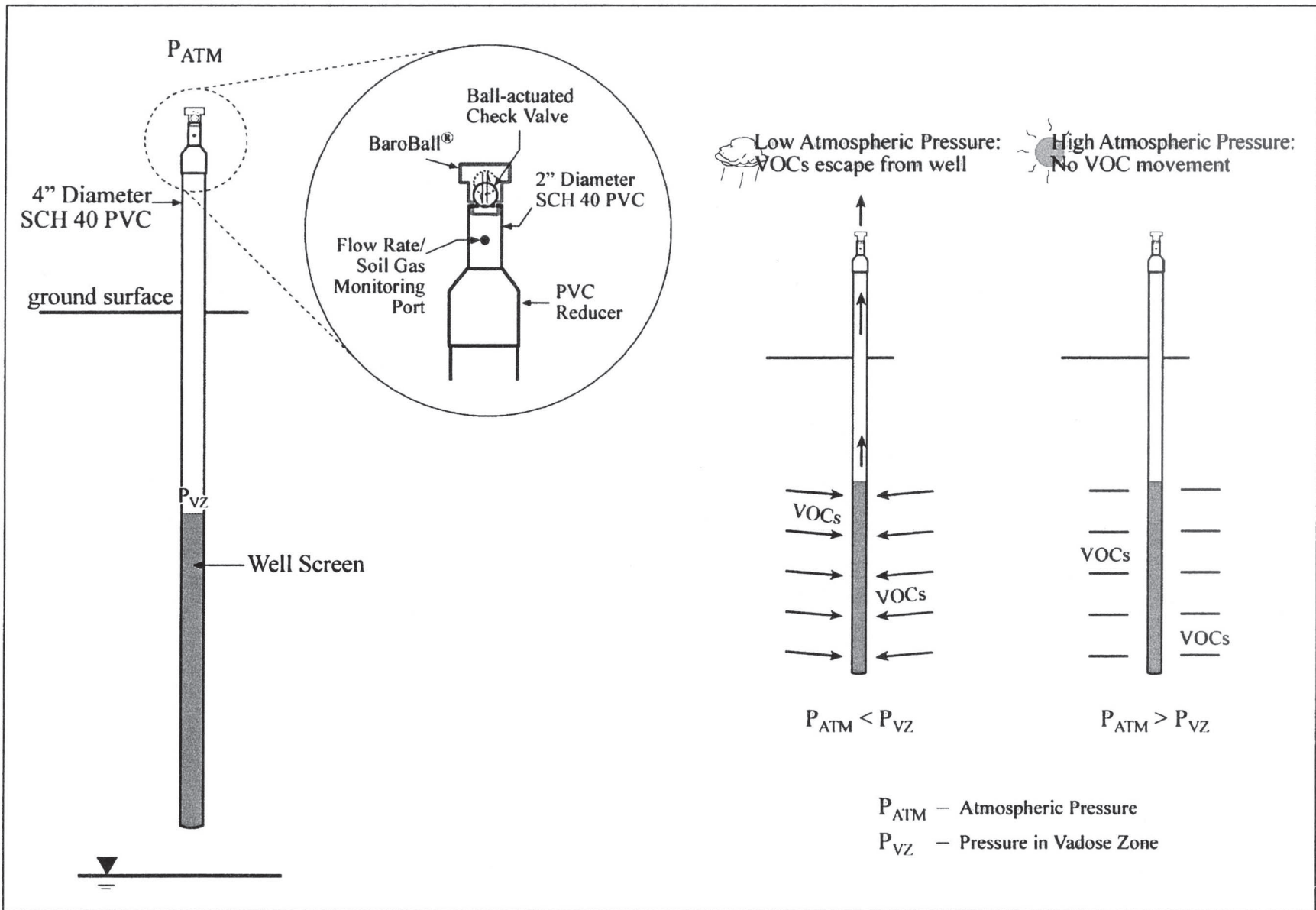
Figure 11 Schematic of Passive Soil-Gas Venting Well Equipped with a BaroBall™ Device Chemical Waste Landfill
