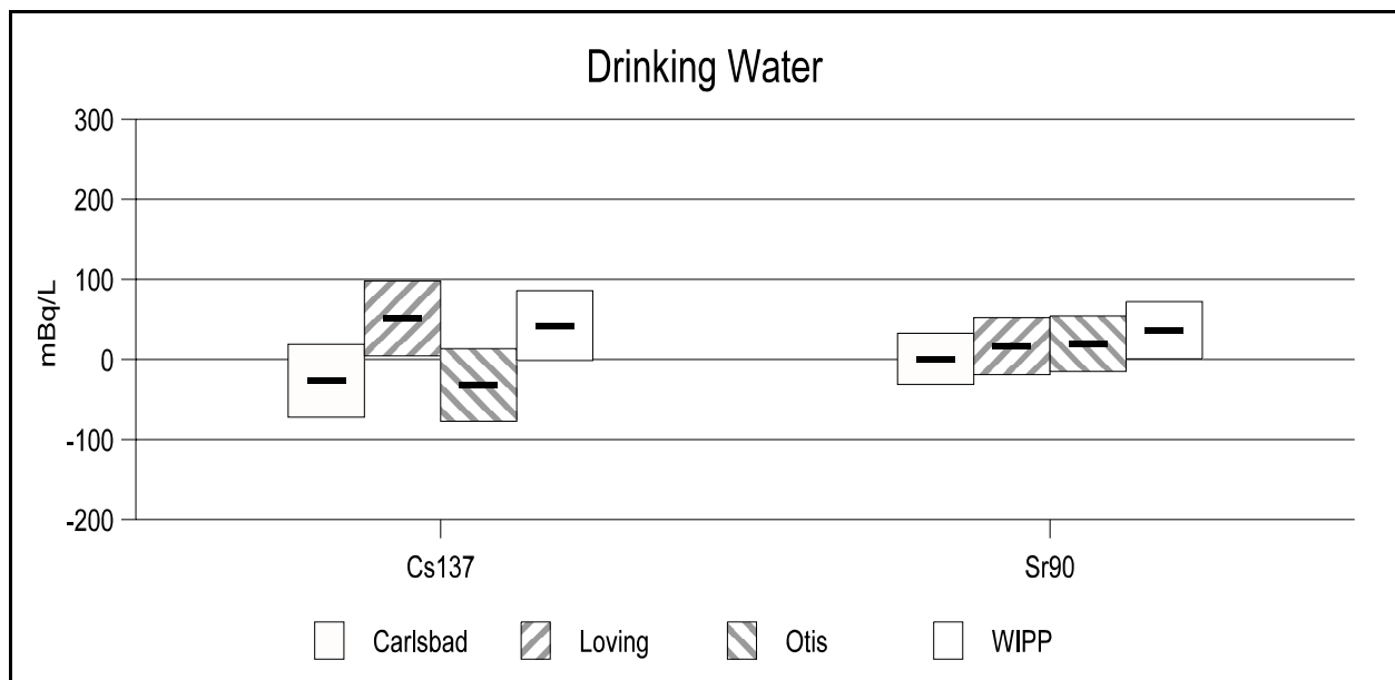
Figure B6. 137 Cs and 90 Sr Measurements in Drinking Water During 2000
