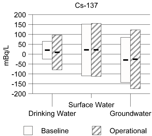
Figure 7. Baseline and 2000 Measurements of 137 Cs in Drinking Water, Surface Water and Groundwater
