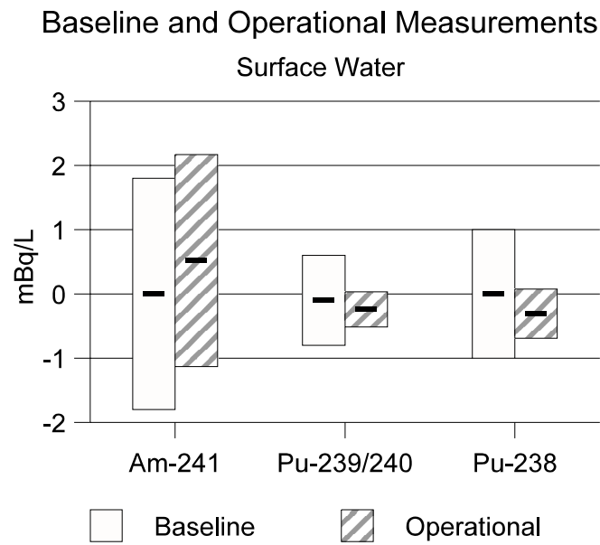
Figure 4. Baseline and 2000 Measurements of ^{241}\text{Am} , ^{239/240}\text{Pu} , and ^{238}\text{Pu} in Surface Water
