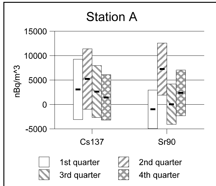
Figure A2. ^{137}\text{Cs} and ^{90}\text{Sr} Measurements in Station A Samples During 2000
