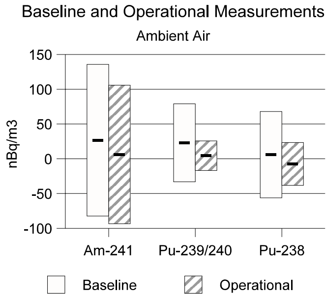
Figure 2. Baseline and 2000 Ambient Air Measurements of ^{241}\text{Am} , ^{239/240}\text{Pu} , and ^{238}\text{Pu}
