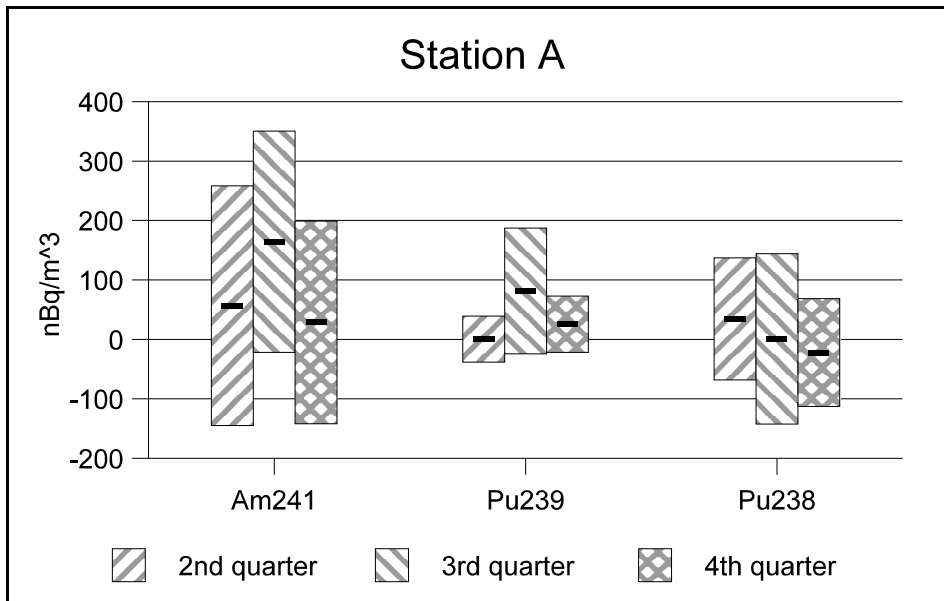
Figure A1. ^{241}\text{Am} , ^{239/240}\text{Pu} , and ^{238}\text{Pu} Measurements in Station A Samples During 2000
