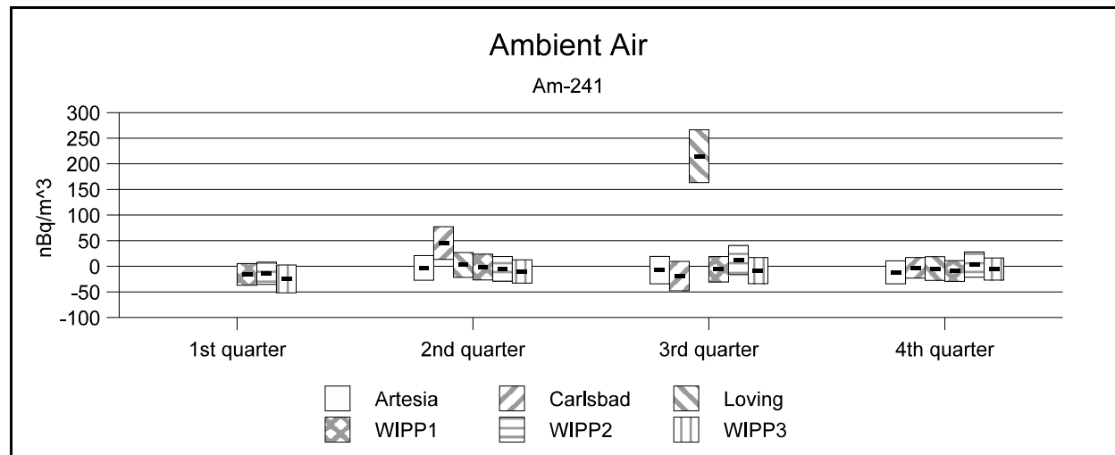
Figure A5. 241 Am Measurements in LVAS Samples During 2000
