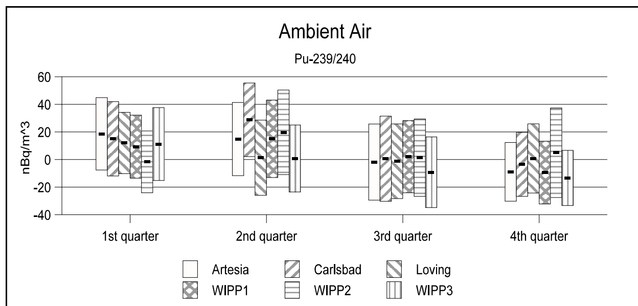
Figure A6. 239/240 Pu Measurements in LVAS Samples During 2000
