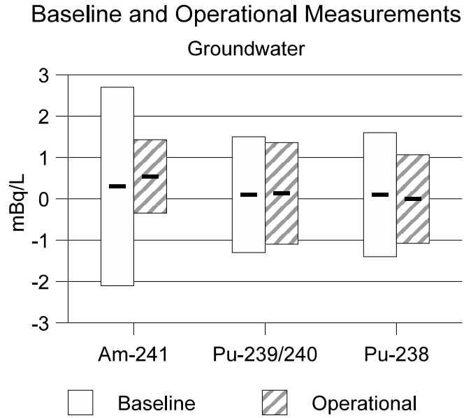
Figure 5. Baseline and 2000 Measurements of ^{241}\text{Am} , ^{239/240}\text{Pu} , and ^{238}\text{Pu} in Groundwater
