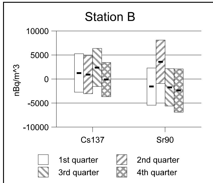
Figure A4. ^{137}\text{Cs} and ^{90}\text{Sr} Measurements in Station B Samples During 2000
