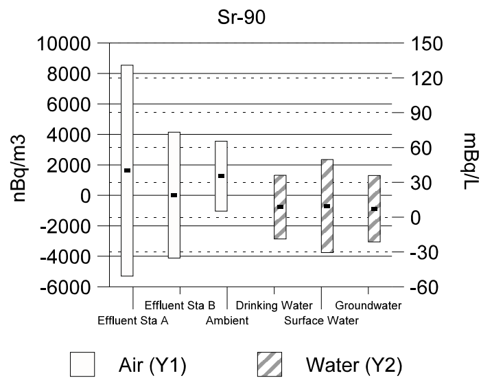
Figure 8. 1999-2000 Measurements of 90 Sr in Air and Water
