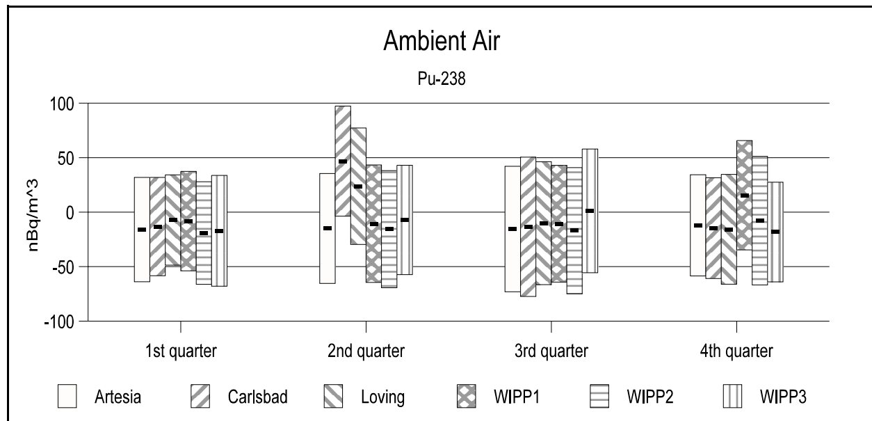
Figure A7. 238 Pu Measurements in LVAS Samples During 2000
