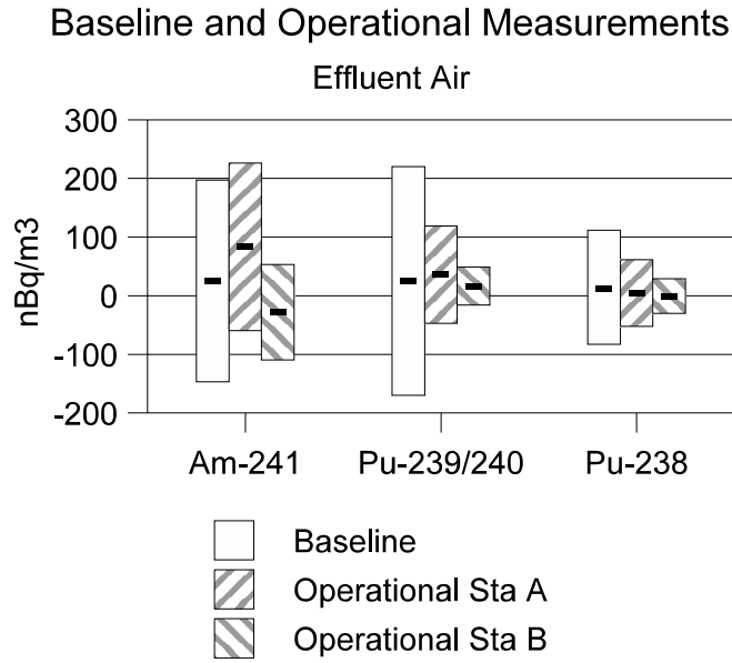
Figure 1. Baseline and 2000 Effluent Air Measurements of ^{241}\text{Am} , ^{239/240}\text{Pu} , and ^{238}\text{Pu}
