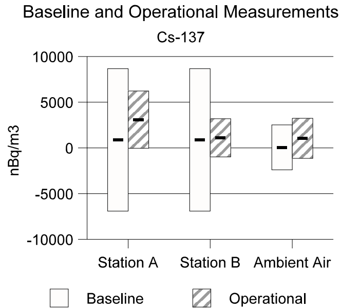
Figure 6. Baseline and 2000 Measurements of ^{137}\text{Cs} in Effluent Air and Ambient Air (Baseline is combined effluent for Stations A and B)
