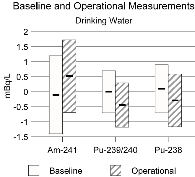
Figure 3. Baseline and 2000 Measurements of ^{241}\text{Am} , ^{239/240}\text{Pu} , and ^{238}\text{Pu} in Drinking Water
