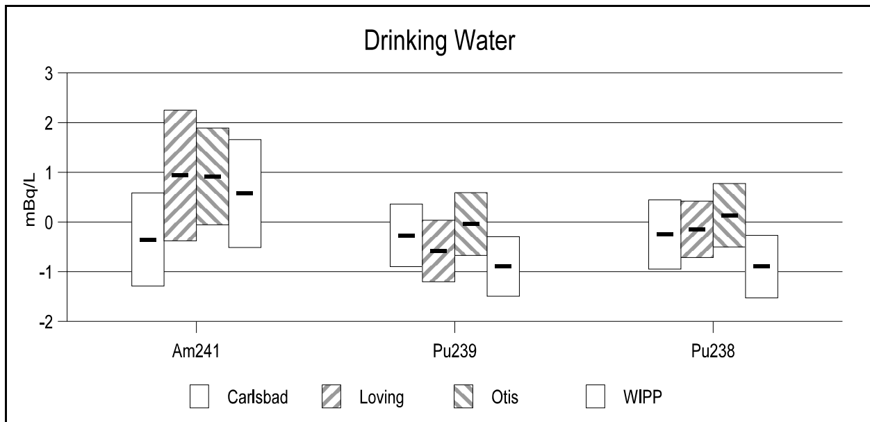
Figure B5. ^{241}\text{Am} , ^{239/240}\text{Pu} , and ^{238}\text{Pu} Measurements in Drinking Water During 2000
