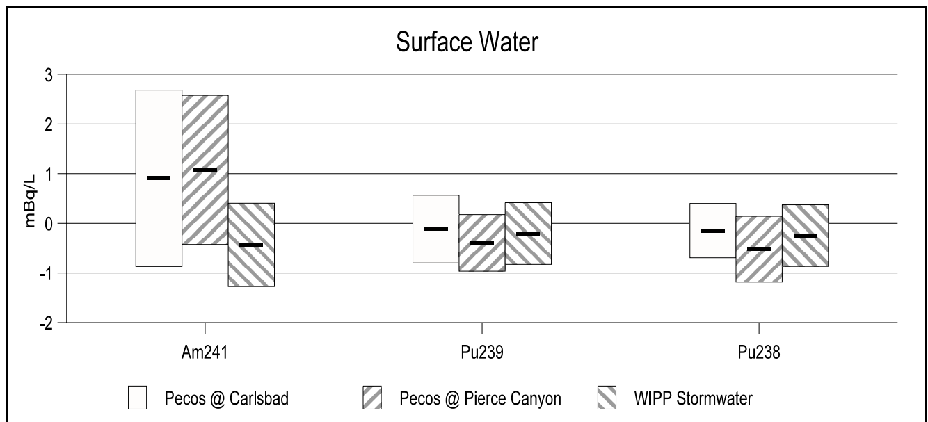
Figure B3. 241 Am, 239/240 Pu, and 238 Pu Measurements in Surface Water During 2000
