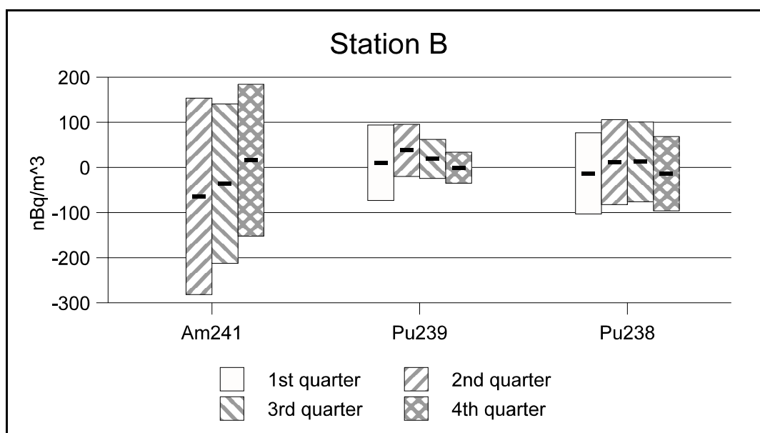
Figure A3. ^{241}\text{Am} , ^{239/240}\text{Pu} , and ^{238}\text{Pu} Measurements in Station B Samples During 2000
