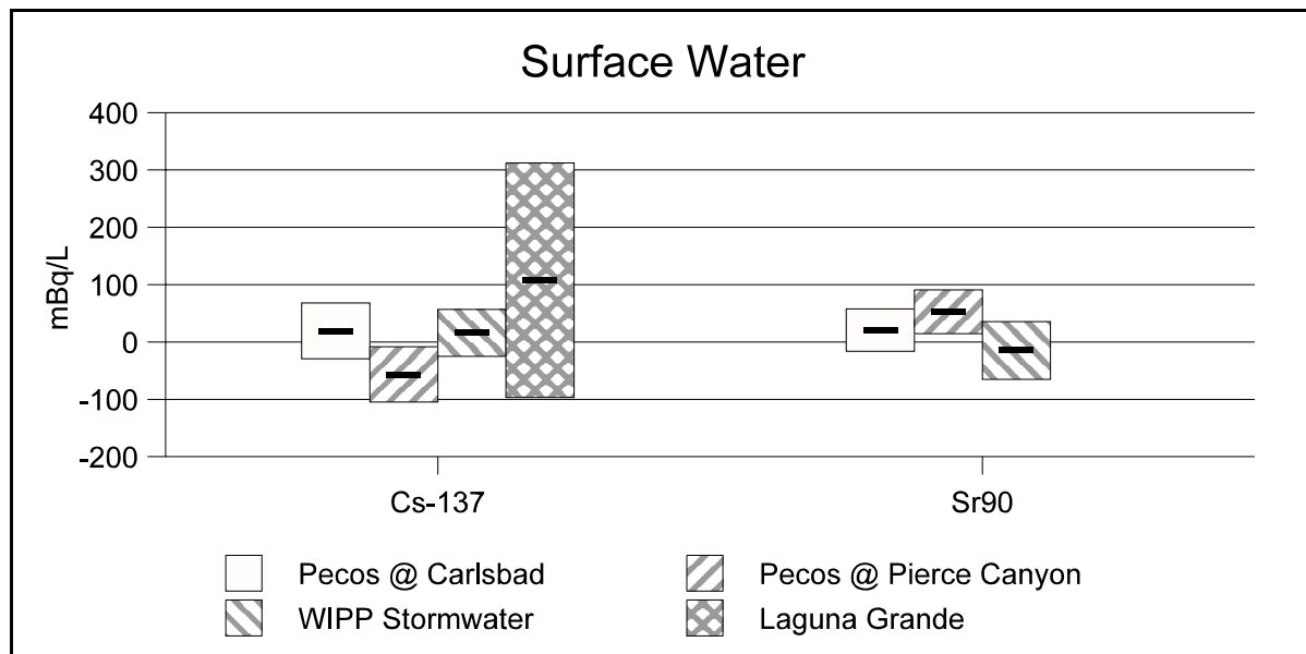
Figure B4. 137 Cs and 90 Sr Measurements in Surface Water During 2000
