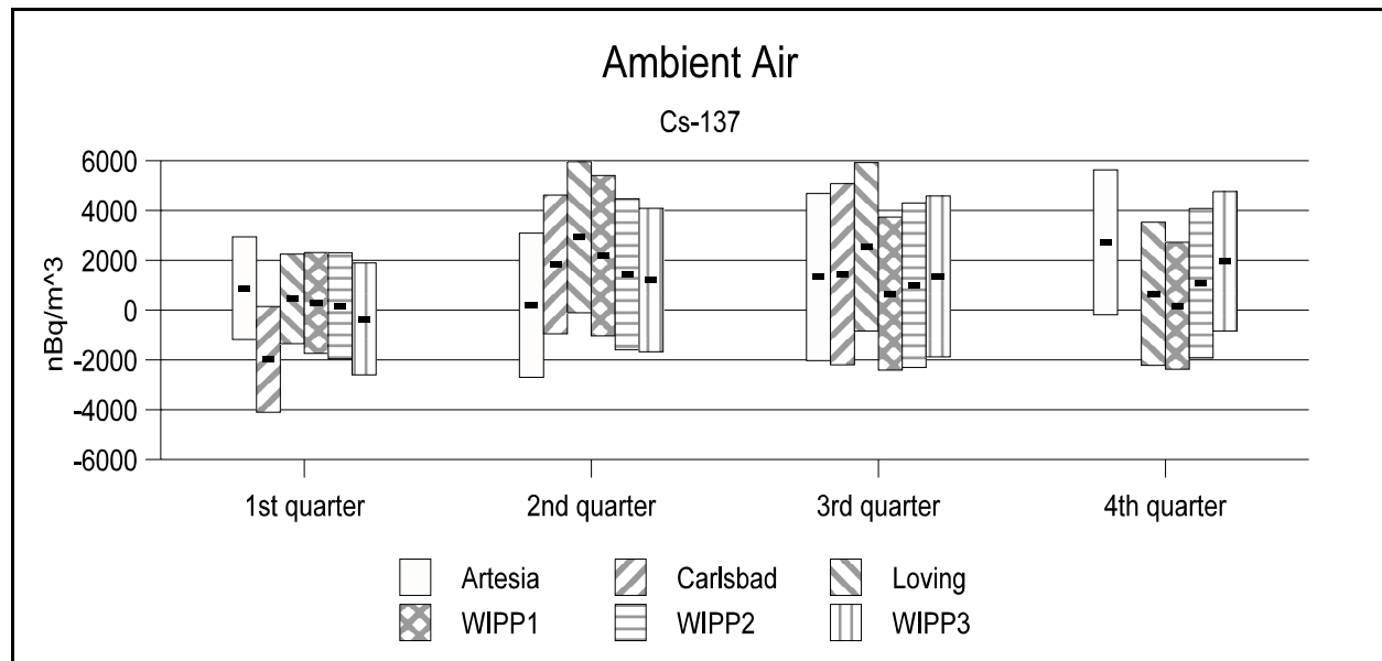
Figure A8. 137 Cs Measurements in LVAS Samples During 2000
