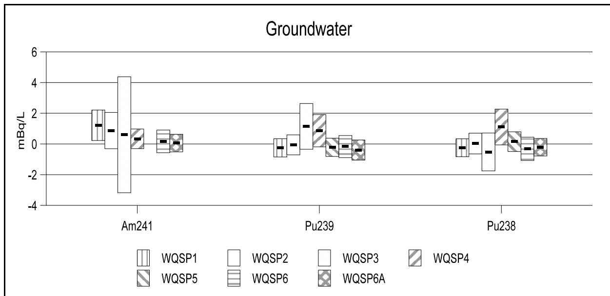
Figure B1. 241 Am, 239/240 Pu, and 238 Pu Measurements in Groundwater During 2000
