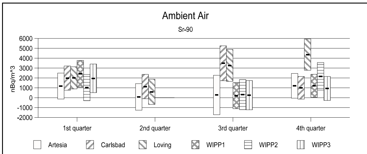
Figure A9. 90 Sr Measurements in LVAS Samples During 2000
