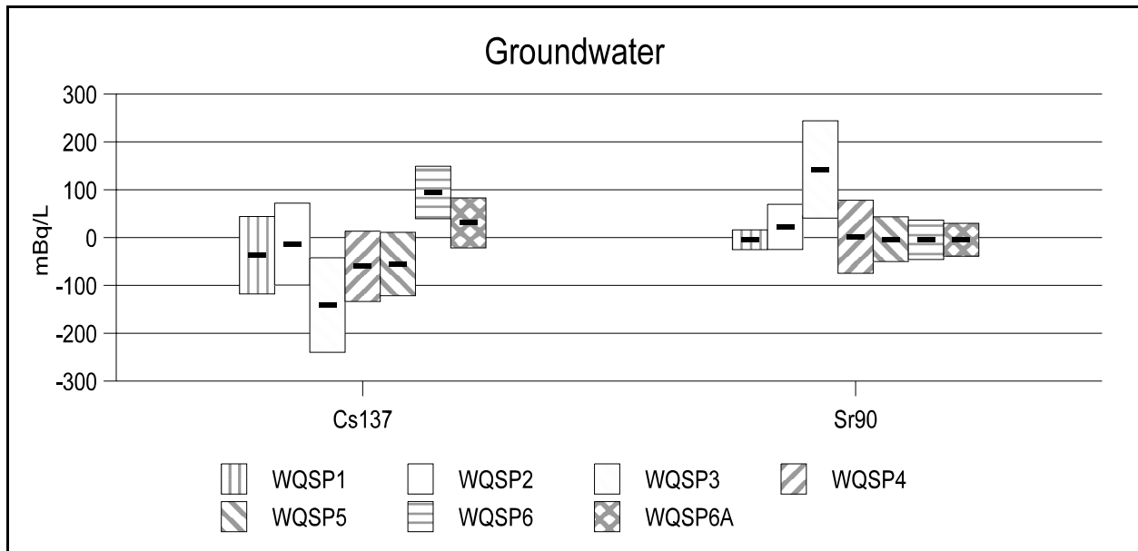
Figure B2. 137 Cs and 90 Sr Measurements in Groundwater During 2000
