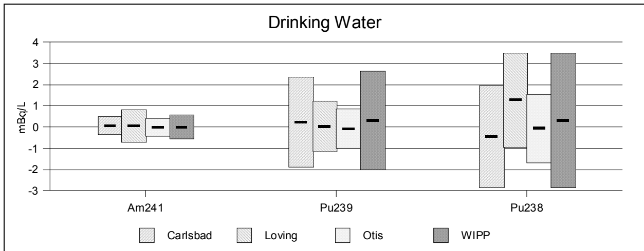
Figure B5. ^{241}\text{Am} , ^{239/240}\text{Pu} , and ^{238}\text{Pu} Measurements in Drinking Water During 2002
