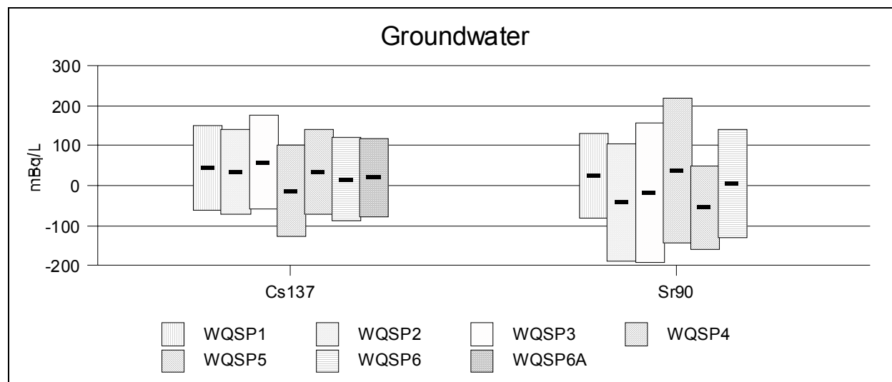
Figure B2. 137 Cs and 90 Sr Measurements in Groundwater During 2002
