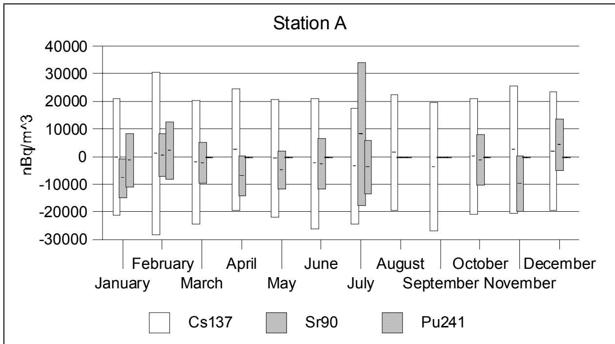
Figure A2. 137 Cs, 90 Sr and 241 Pu Measurements in Station A Samples During 2002
