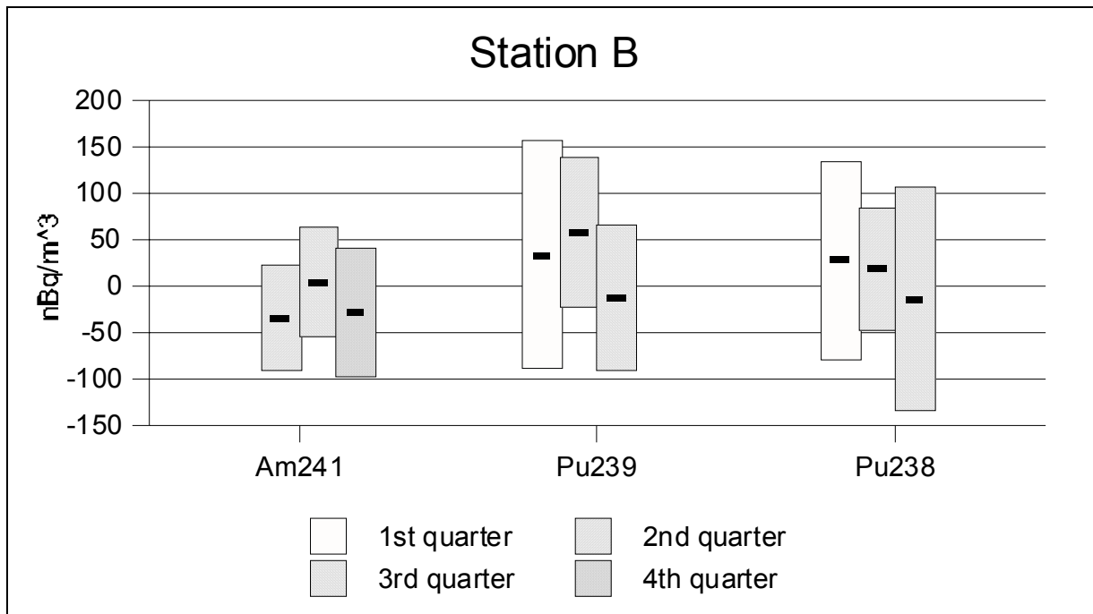
Figure A3. ^{241}\text{Am} , ^{239/240}\text{Pu} , and ^{238}\text{Pu} Measurements in Station B Samples During 2002
