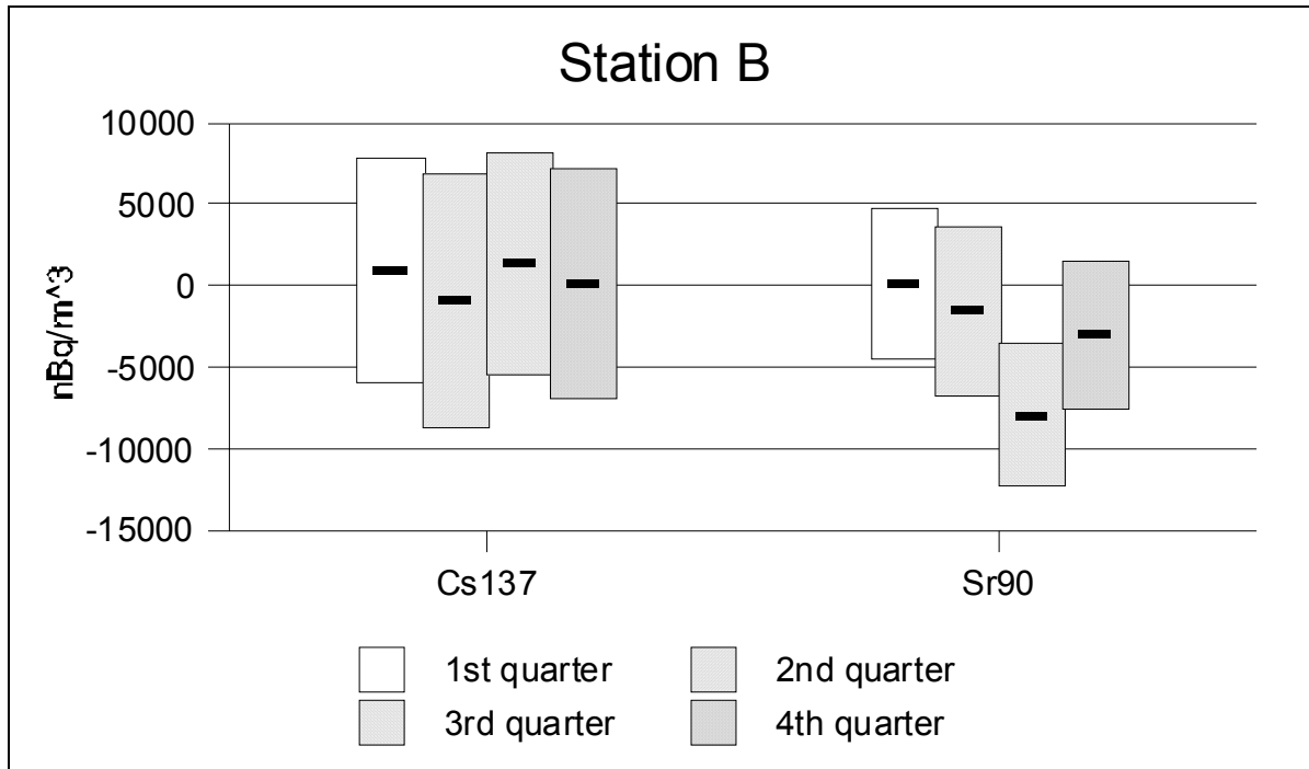
Figure A4. 137 Cs and 90 Sr Measurements in Station B Samples During 2002
