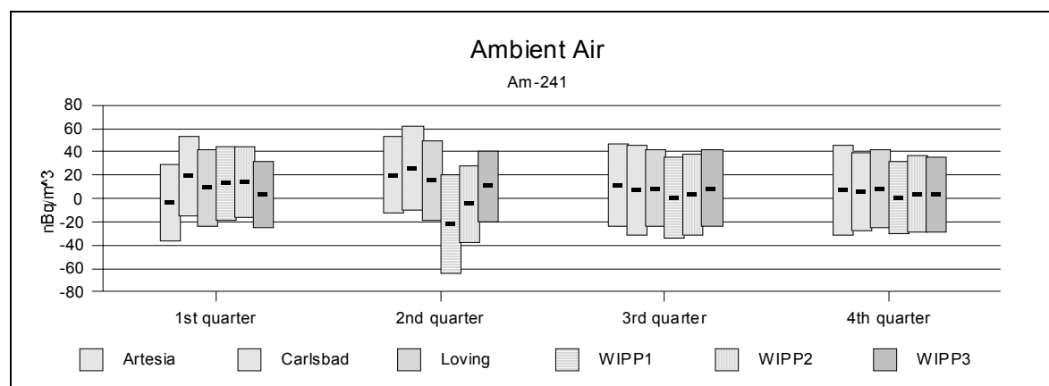
Figure A5. 241 Am Measurements in LVAS Samples During 2002
