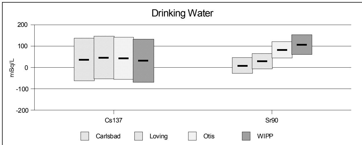
Figure B6. 137 Cs and 90 Sr Measurements in Drinking Water During 2002
