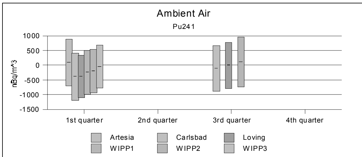
Figure A8. 241 Pu Measurements in LVAS Samples During 2002
