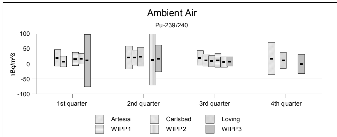
Figure A6. 239/240 Pu Measurements in LVAS Samples During 2002
