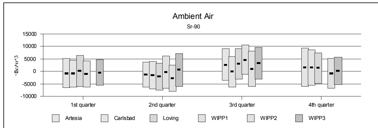
Figure A10. 90 Sr Measurements in LVAS Samples During 2002
