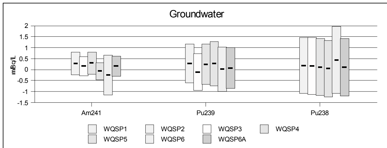
Figure B1. ^{241}\text{Am} , ^{239/240}\text{Pu} , and ^{238}\text{Pu} Measurements in Groundwater During 2002
