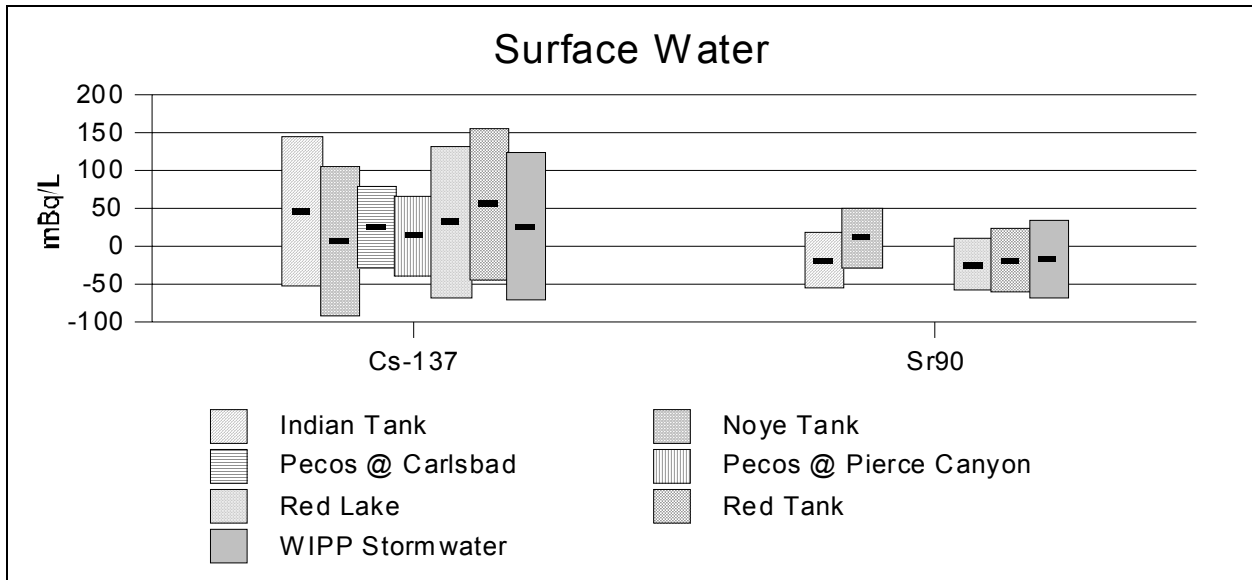
Figure B4. 137 Cs and 90 Sr Measurements in Surface Water During 2002
