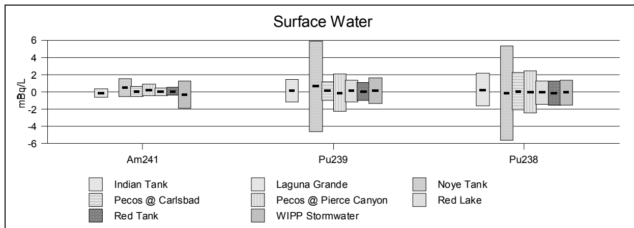
Figure B3. ^{241}\text{Am} , ^{239/240}\text{Pu} , and ^{238}\text{Pu} Measurements in Surface Water During 2002
