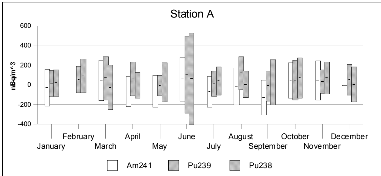
Figure A1. ^{241}\text{Am} , ^{239/240}\text{Pu} , and ^{238}\text{Pu} Measurements in Station A Samples During 2002
