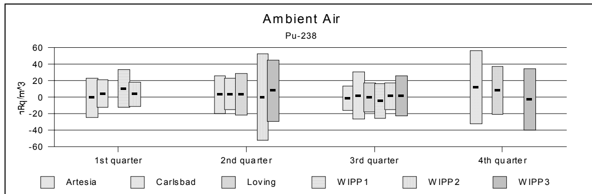
Figure A7. 238 Pu Measurements in LVAS Samples During 2002
