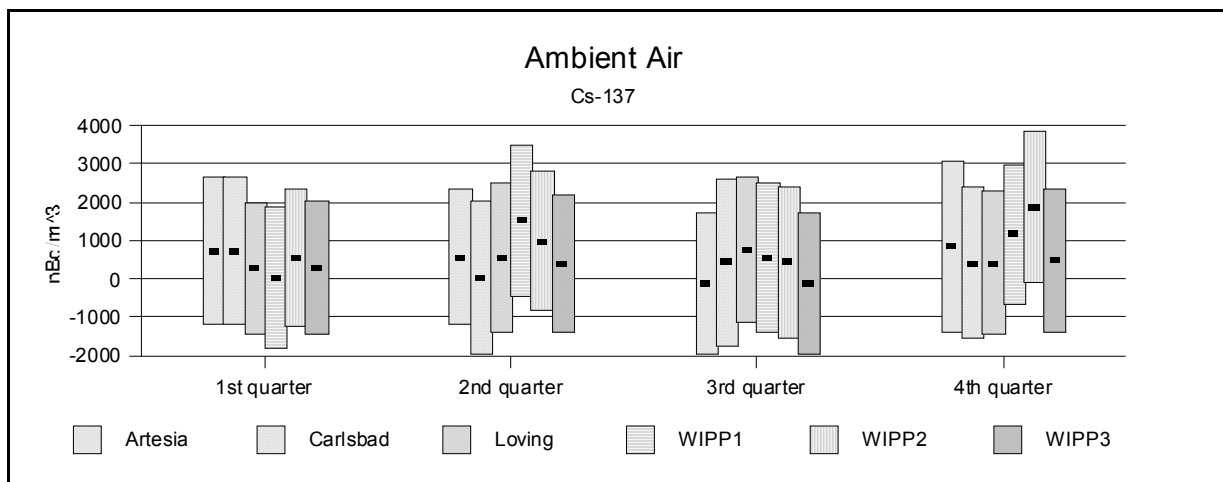
Figure A9. 137 Cs Measurements in LVAS Samples During 2002
