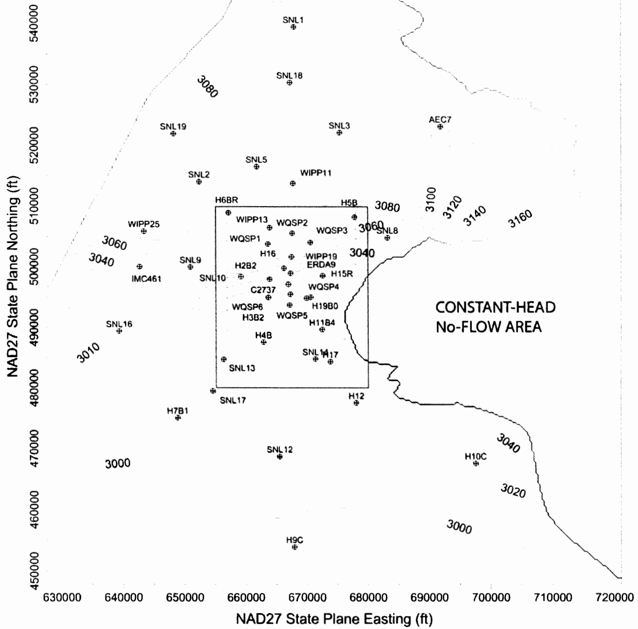
Figure 1 – Model-Generated June 2009 Freshwater Head Contours in the Model Domain (Contour Interval = 10 feet amsl)
