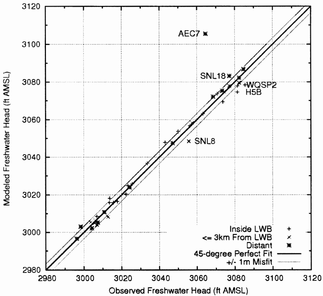
Figure 3 – Measured Versus Modeled Scatter Plot for PEST-Calibrated MODFLOW-2000 Generated Heads and June 2009 Observed Freshwater Heads
