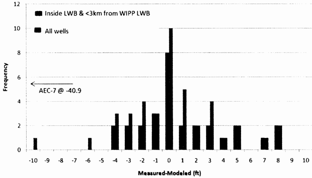
Figure 4 - Frequency of Modeled Freshwater Head Residuals
