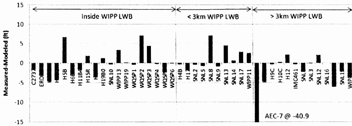
Figure 5 - Modeled Residual Freshwater Head at Each Well
