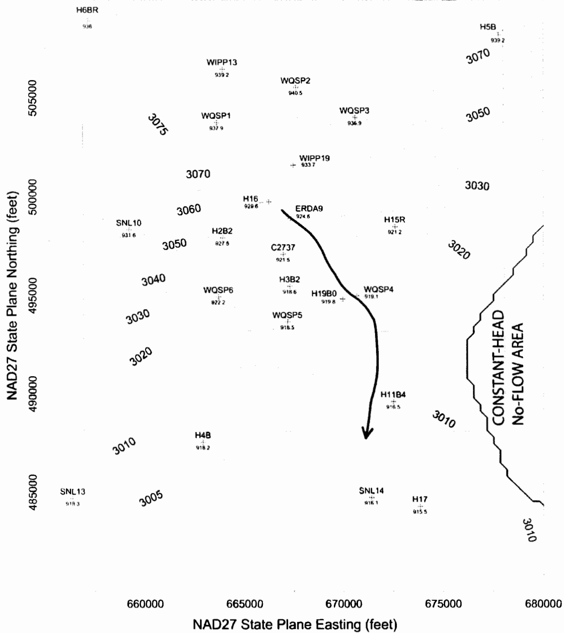
Figure 2 – Model-Generated June 2009 Freshwater Head Contours ( 5-foot Contour Interval) in the WIPP Vicinity with Blue Water Particle Track From Waste Shaft to WIPP LWB
