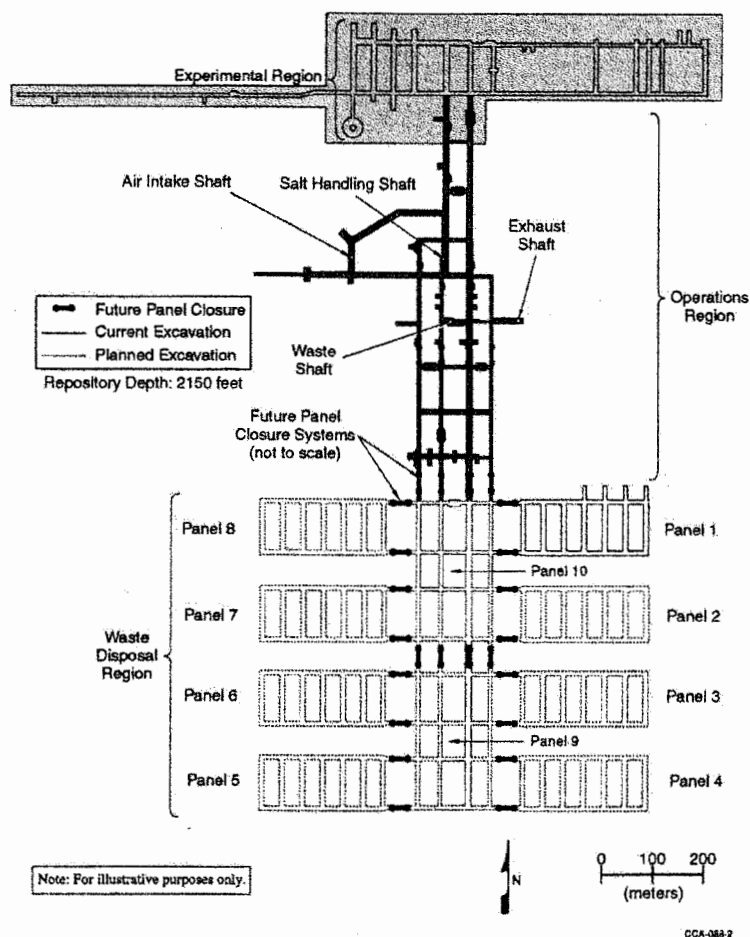
Figure 3-2. Plan View of WIPP Underground Facility and Panel Closure Systems
