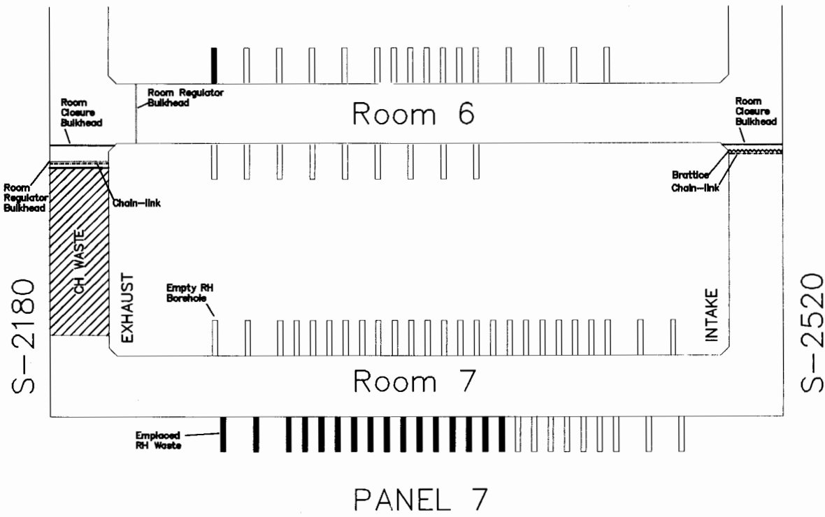
Figure 4 Proposed Location for Bulkheads that will Close Panel 7, Room 7
