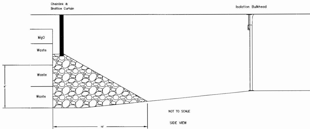
Figure 2 Typical Layout for the Initial Closure in Panel 6
