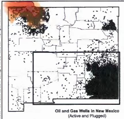
Methane Hotspot Source: NASA & University of Michigan, October 9, 2014
