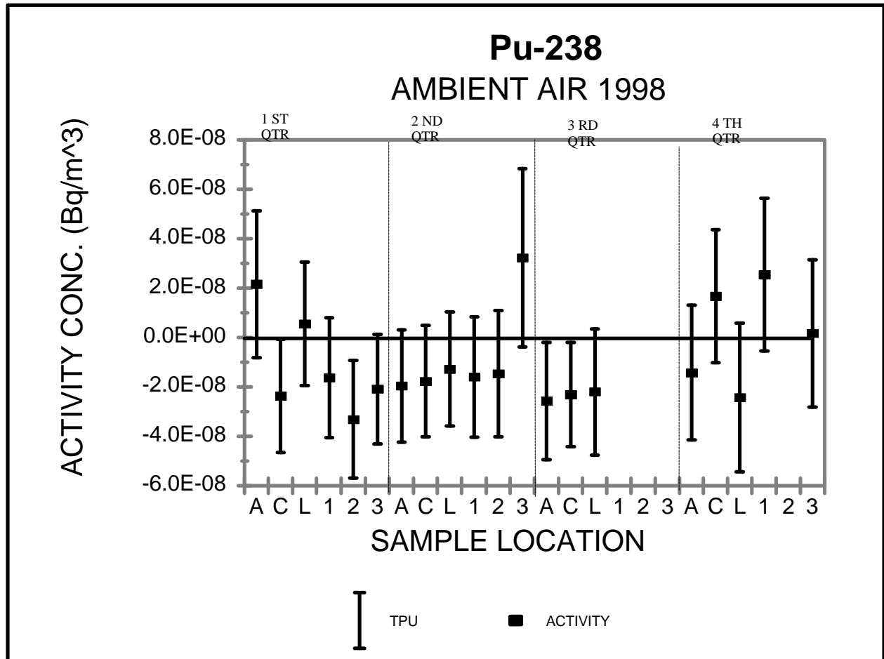
Figure B3. 238 Pu Concentrations in LVAS Samples During 1998
