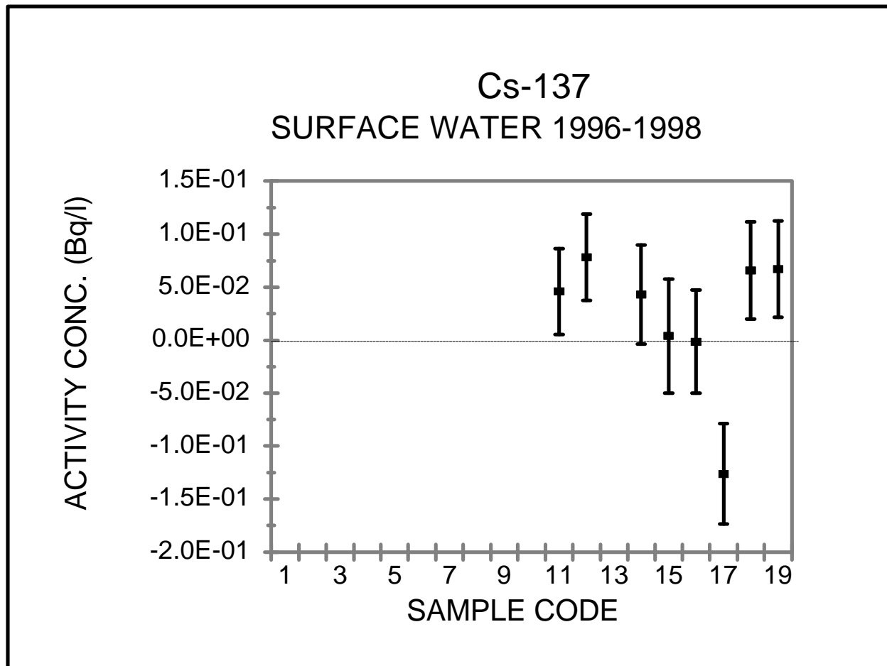
Figure C8. 137 Cs Concentrations in Surface Water During 1996-1998
