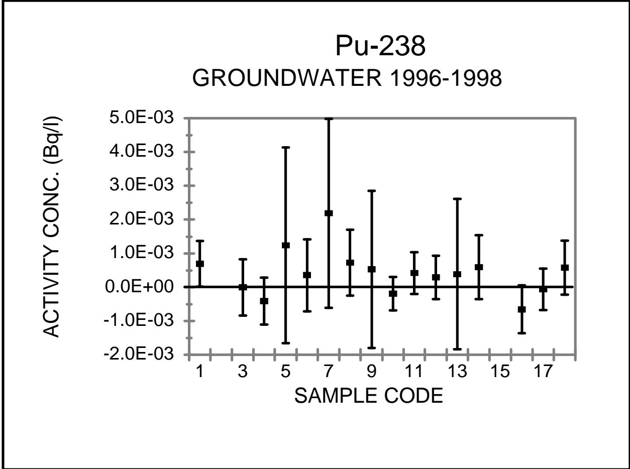
Figure C11. 238 Pu Concentrations in Ground Water During 1996-1998
