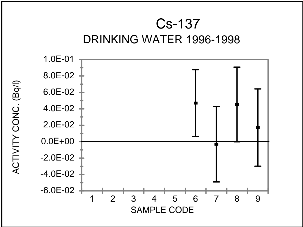
Figure C4. 137 Cs Concentrations in Public Water Systems During 1996-1998
