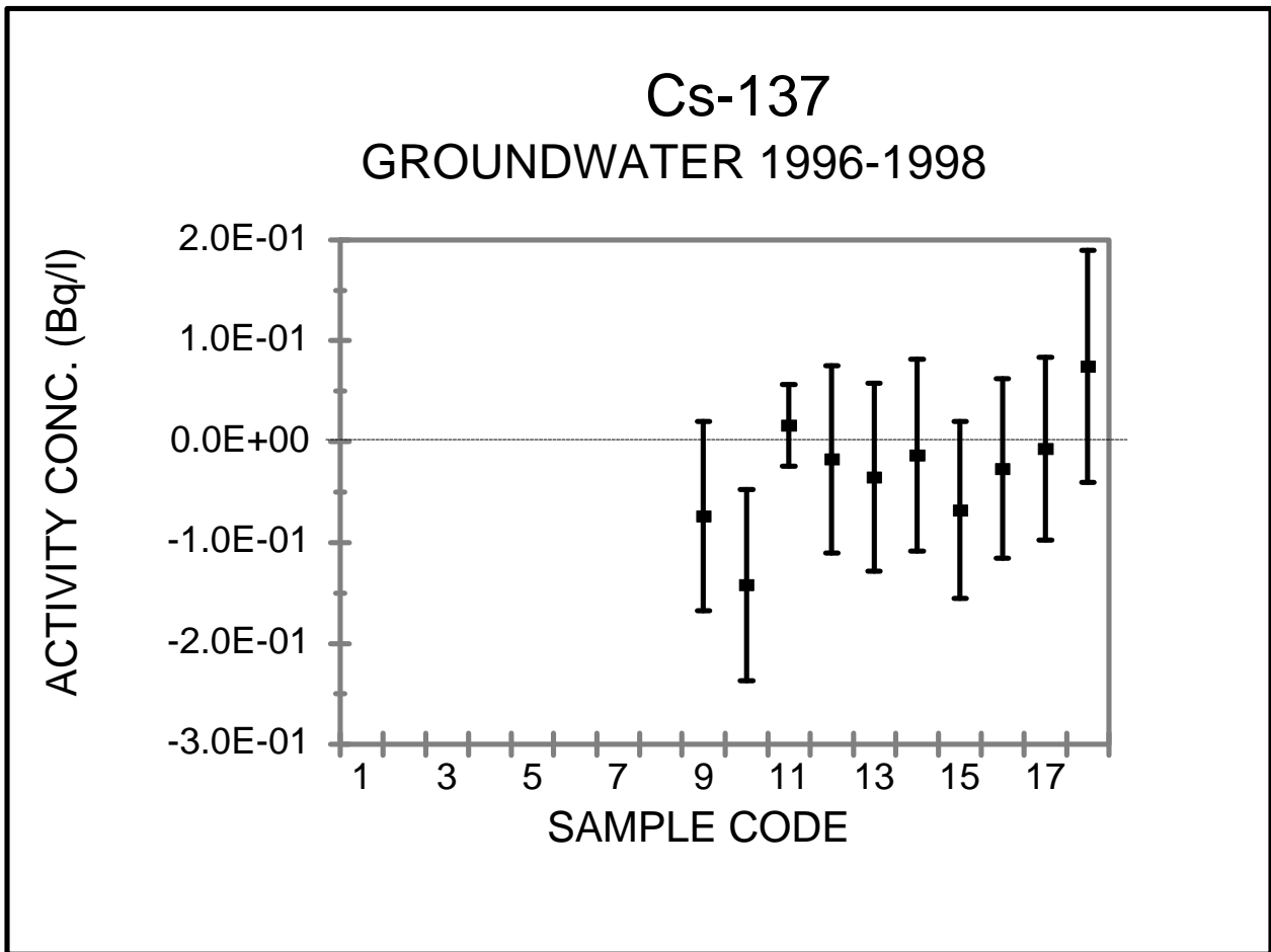
Figure C12. 137 Cs Concentrations in Ground Water During 1996-1998
