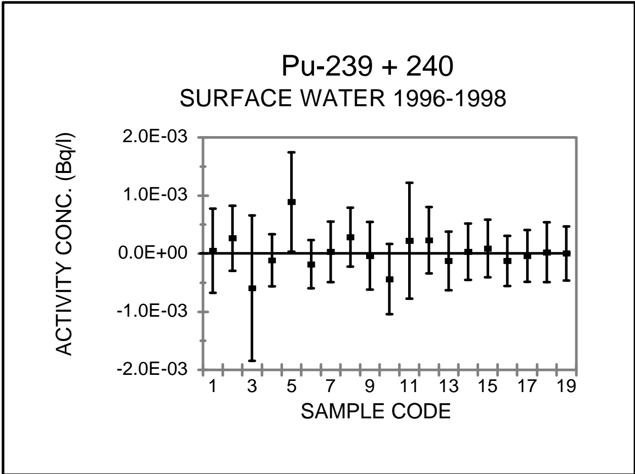
Figure C6. 239+240 Pu Concentrations in Surface Water During 1996-1998
