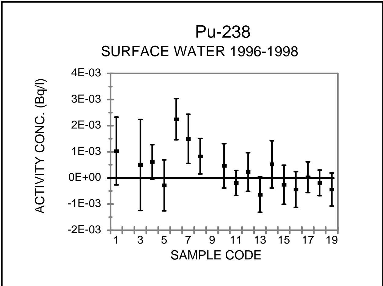
Figure C7. 238 Pu Concentrations in Surface Water During 1996-1998
