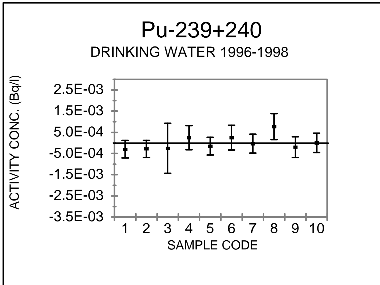
Figure C2. 239+240 Pu Concentrations in Public Water Systems During 1996-1998
