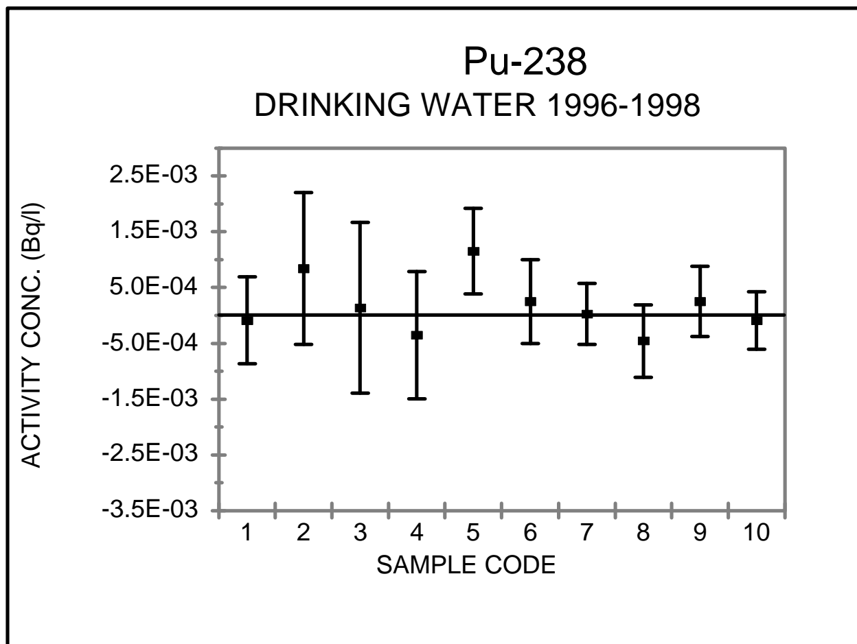
Figure C3. 238 Pu Concentrations in Public Water Systems During 1996-1998
