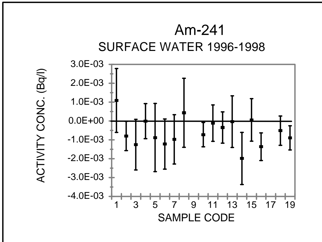
Figure C5. 241 Am Concentrations in Surface Water During 1996-1998
