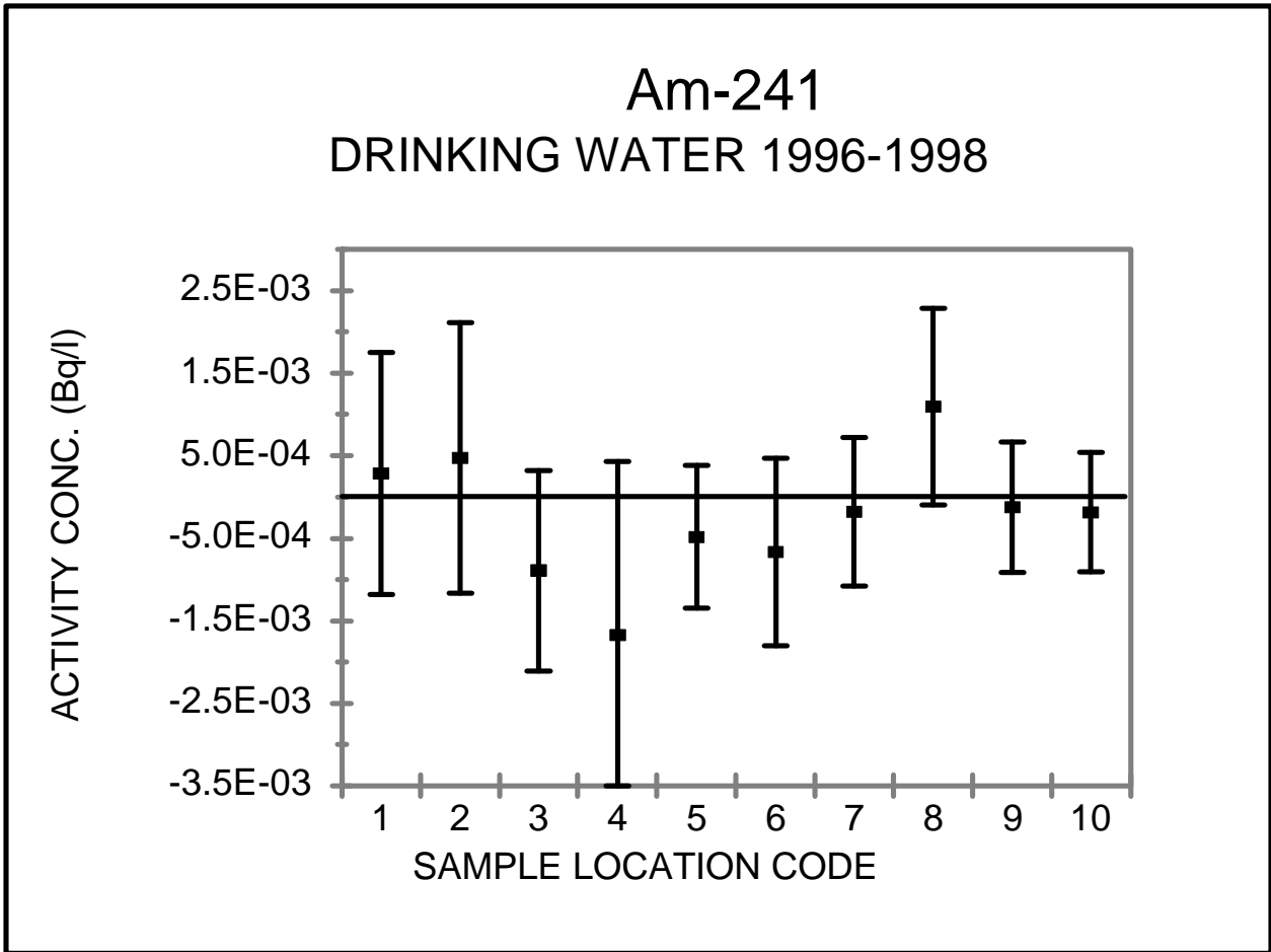
Figure C1. 241 Am Concentrations in Public Water Systems During 1996-1998
