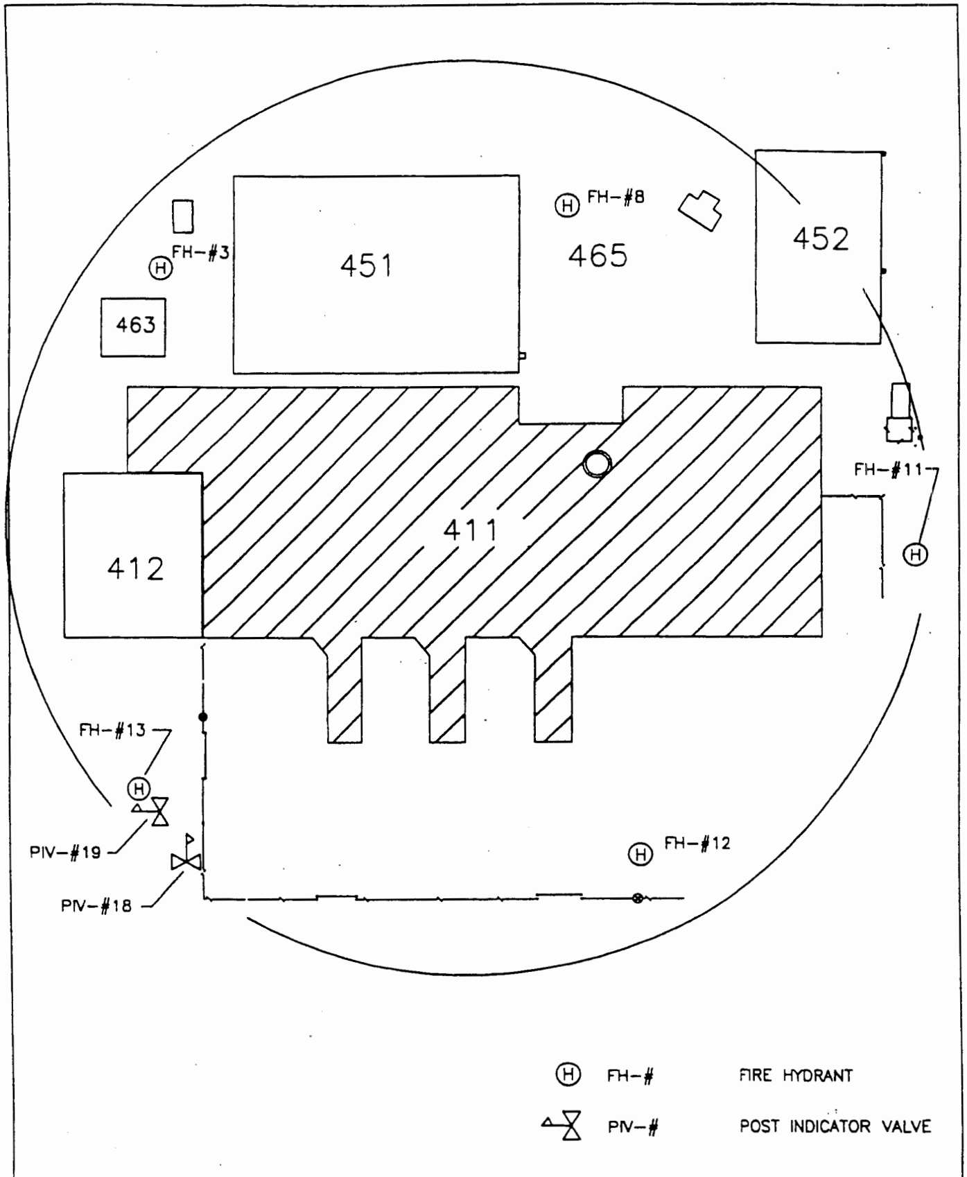
Figure F-10a. Waste Handling Building Pre-Fire Survey (First Floor - Fire Hydrant/Post Indicator Location)
